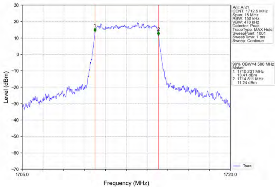
Band66_5MHz_QPSK_LCH_1712.5MHz_RB_25_0_NTNV
