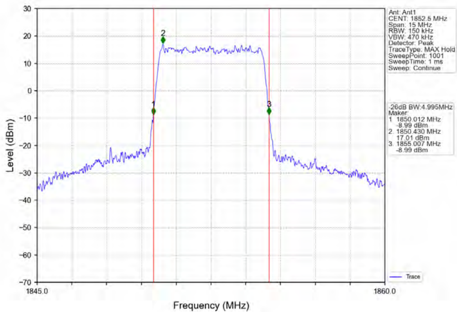
Band2_5MHz_64QAM_LCH_1852.5MHz_RB_25_0_NTNV
