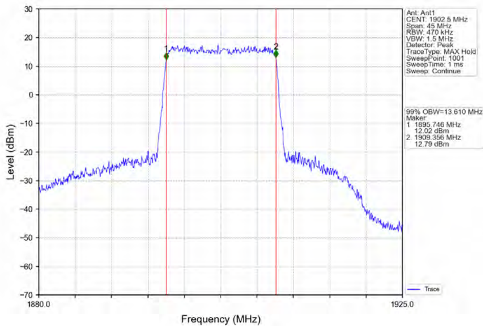
Band2_15MHz_64QAM_HCH_1902.5MHz_RB_75_0_NTNV
