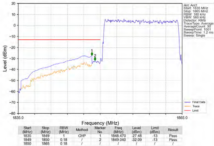
Band2_15MHz_QPSK_LCH_1857.5MHz_RB_75_0_NTNV
