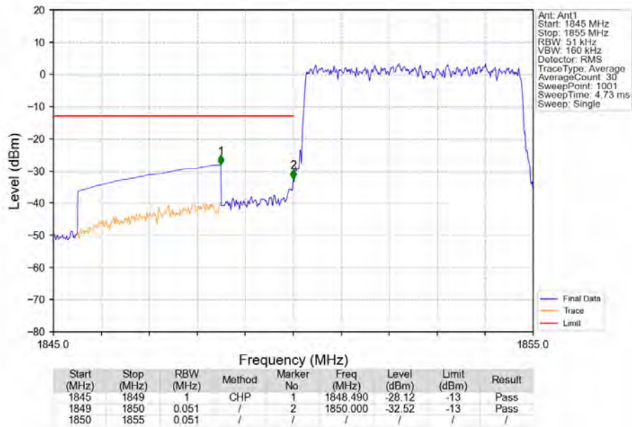
Band2_5MHz_64QAM_LCH_1852.5MHz_RB_25_0_NTNV
