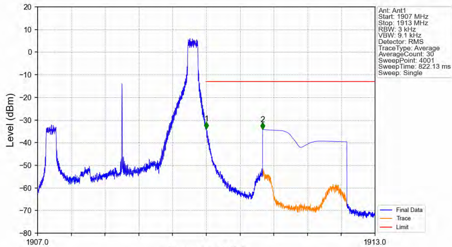
Band2_3MHz_64QAM_HCH_1908.5MHz_RB_1_14_NTNV
