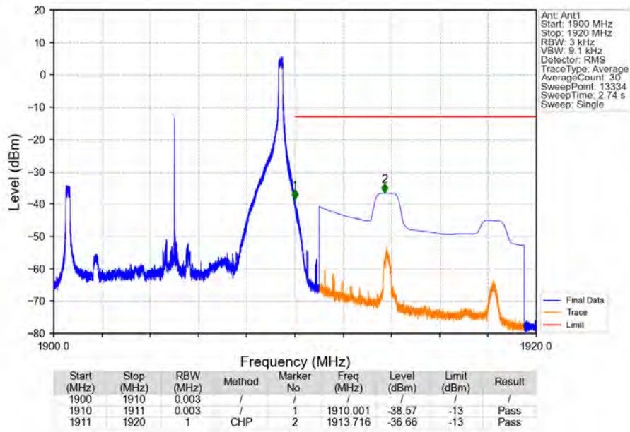
Band2_10MHz_64QAM_HCH_1905MHz_RB_1_49_NTNV
