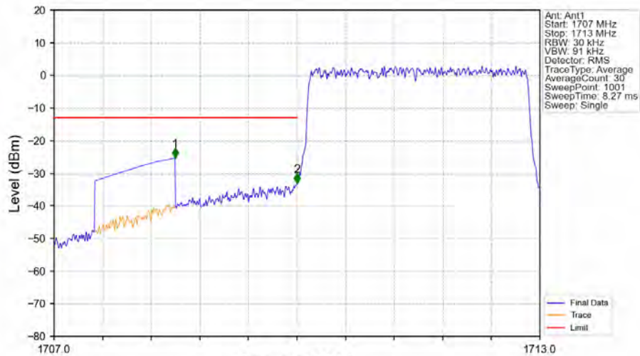
Band4_3MHz_64QAM_LCH_1711.5MHz_RB_15_0_NTNV
