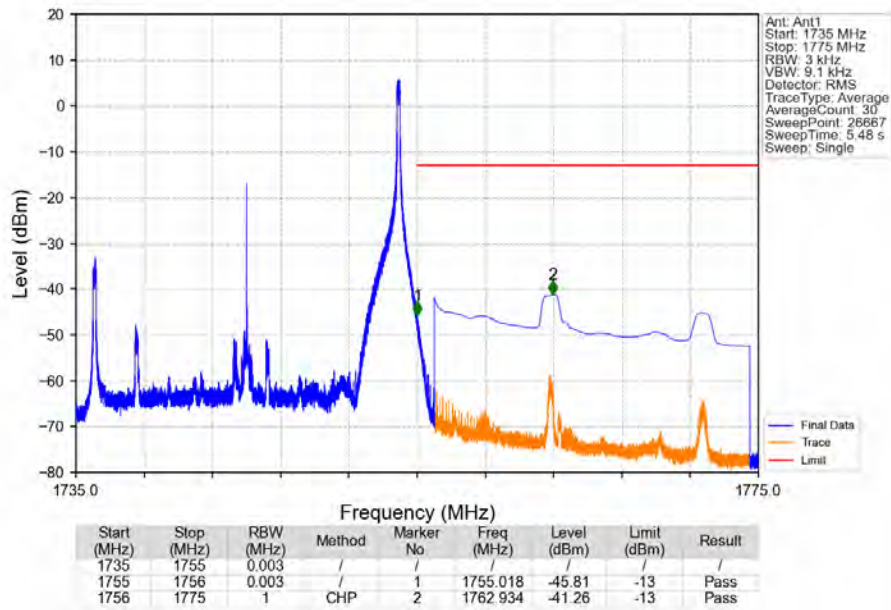
Band4_20MHz_64QAM_HCH_1745MHz_RB_1_99_NTNV
