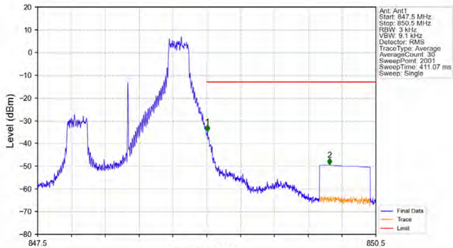
Band5_1.4MHz_16QAM_HCH_848.3MHz_RB_1_5_NTNV
