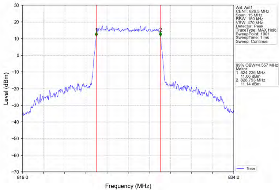
Band5_5MHz_QPSK_LCH_826.5MHz_RB_25_0_NTNV
