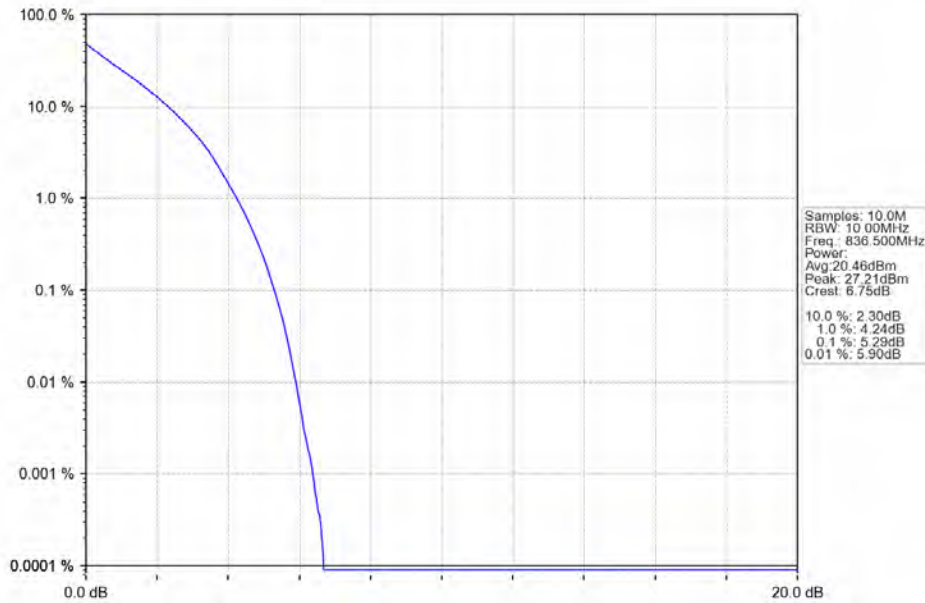
Band5_10MHz_QPSK_MCH_836.5MHz_RB_50_0_NTNV
