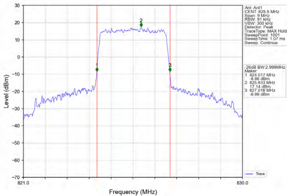
Band5_3MHz_QPSK_LCH_825.5MHz_RB_15_0_NTNV
