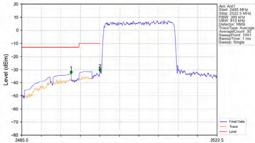
Band7_15MHz_QPSK_LCH_2507.5MHz_RB_75_0_NTNV
