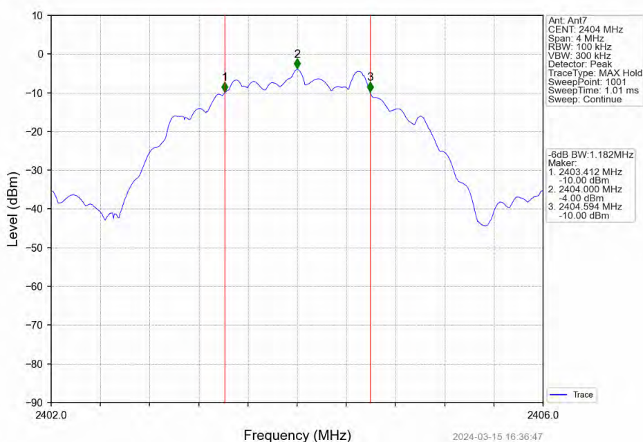
2M_LCH_2404MHz_Ant7_NTNV
