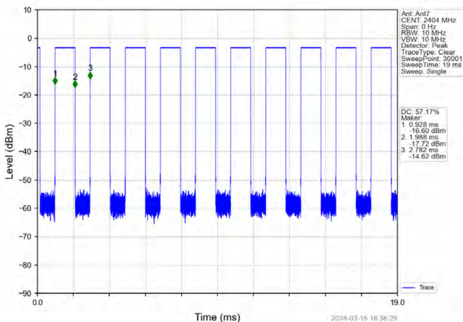
2M_LCH_2404MHz_Ant7_NTNV
