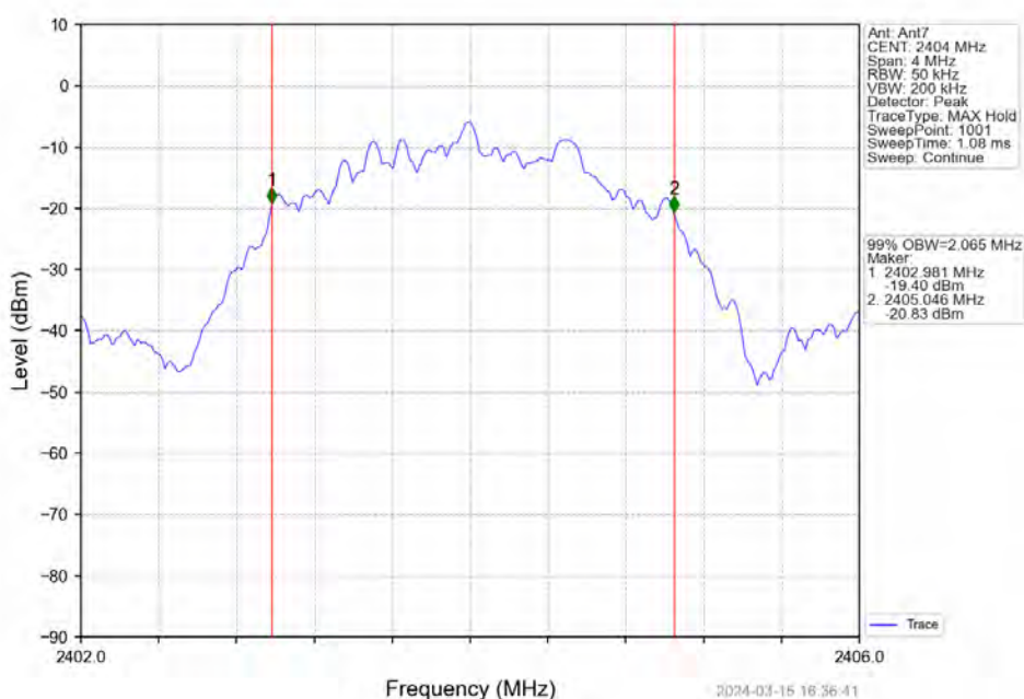
2M_LCH_2404MHz_Ant7_NTNV
