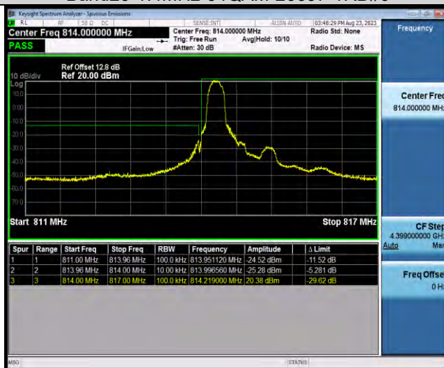
Band26-1.4MHz-64QAM-26697-6RB#0
