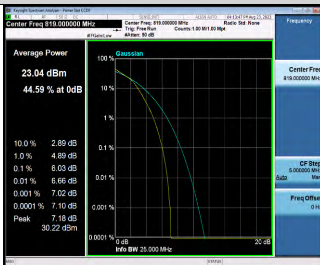
Band26-10MHz-64QAM-26740-1RB#0
