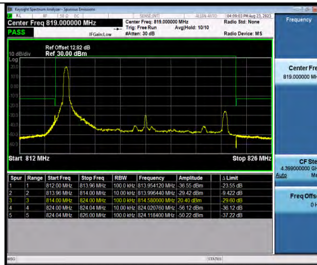
Band26-10MHz-16QAM-26740-1RB#49
