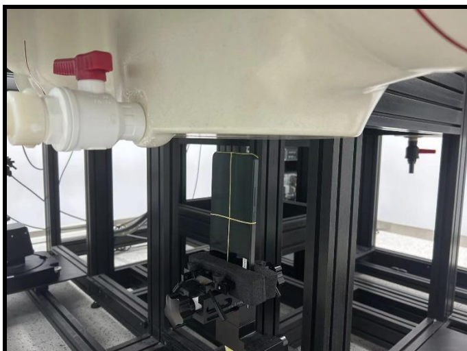
Top Side of EUT with 1.9 cm Gap
