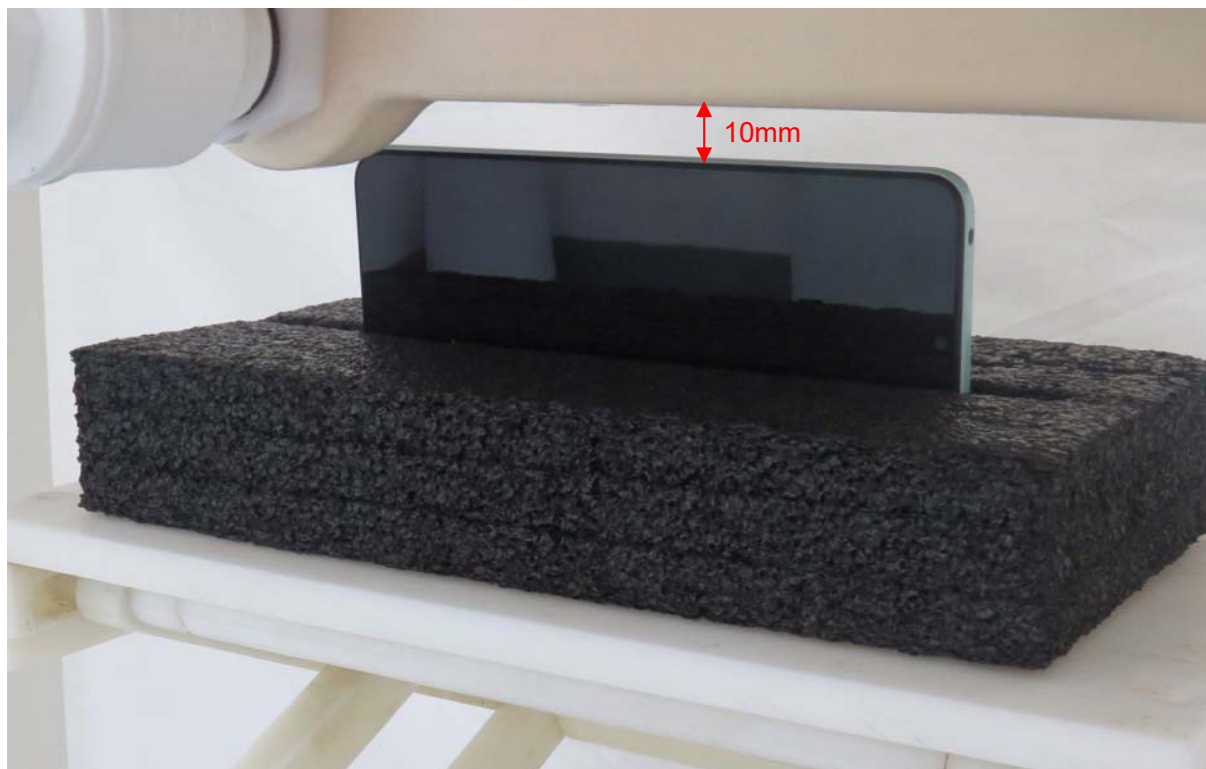
Picture 7: Left Edge, the distance from handset to the bottom of the Phantom is 10mm
