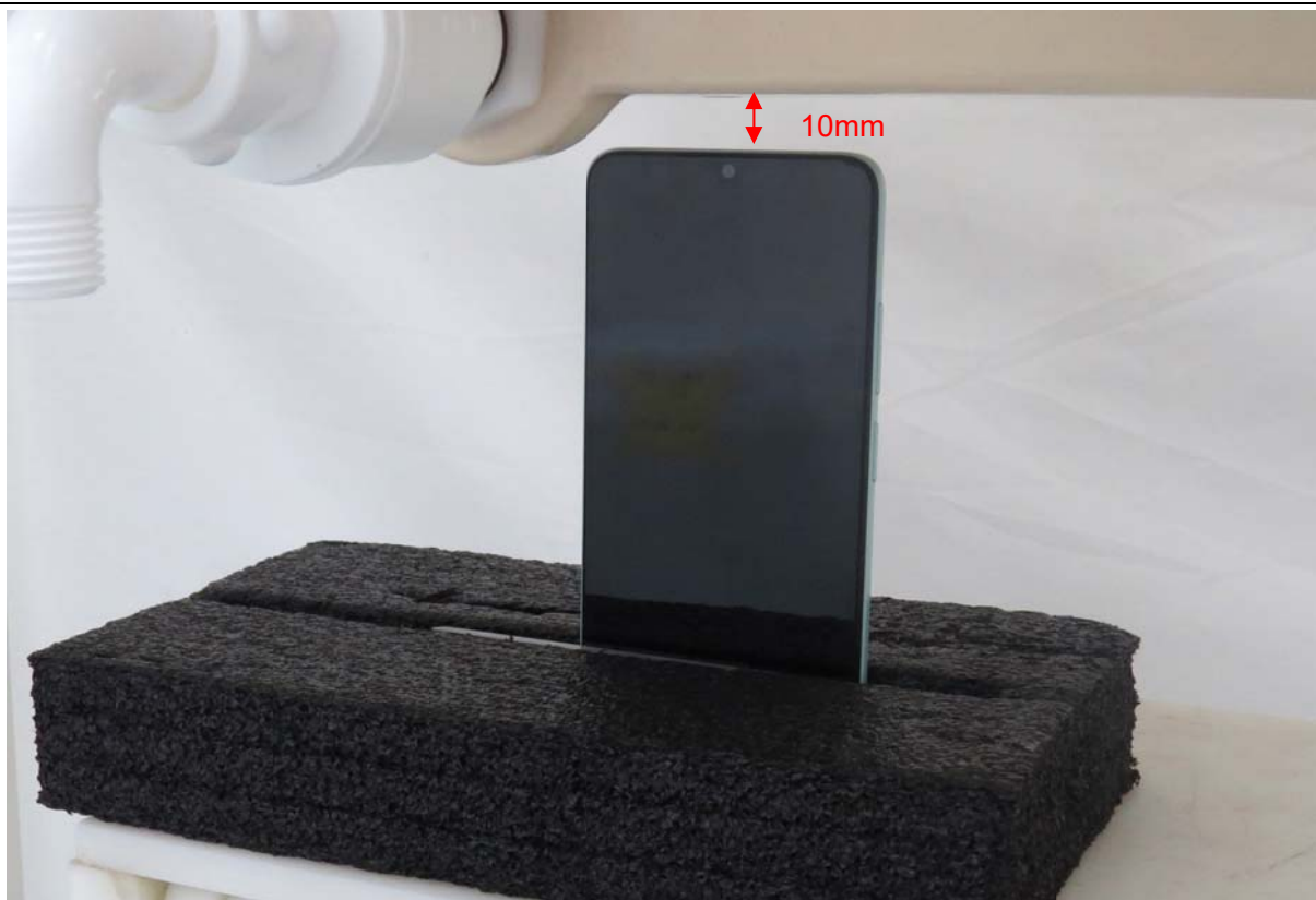
Picture 9: Top Edge, the distance from handset to the bottom of the Phantom is 10mm
