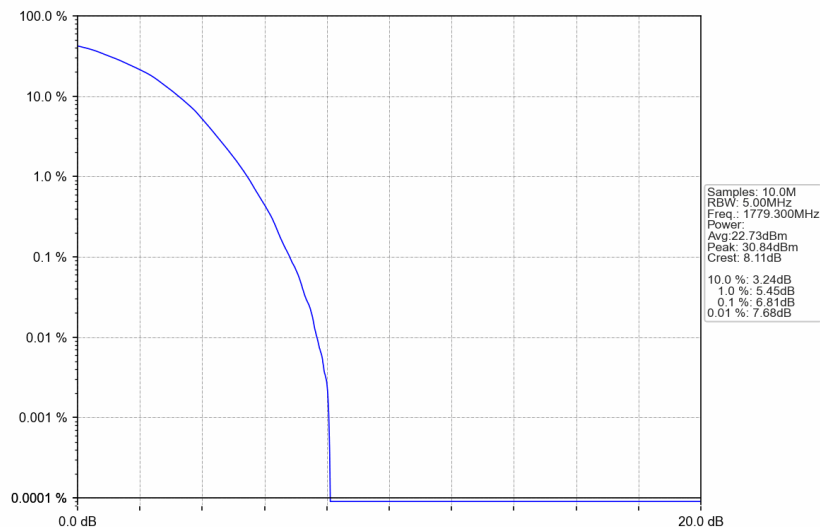
Band66_1.4MHz_64QAM_HCH_1779.3MHz_RB_6_0_NTNV
