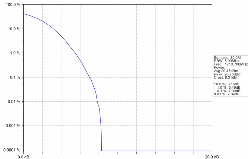
Band66_1.4MHz_256QAM_LCH_1710.7MHz_RB_6_0_NTNV
