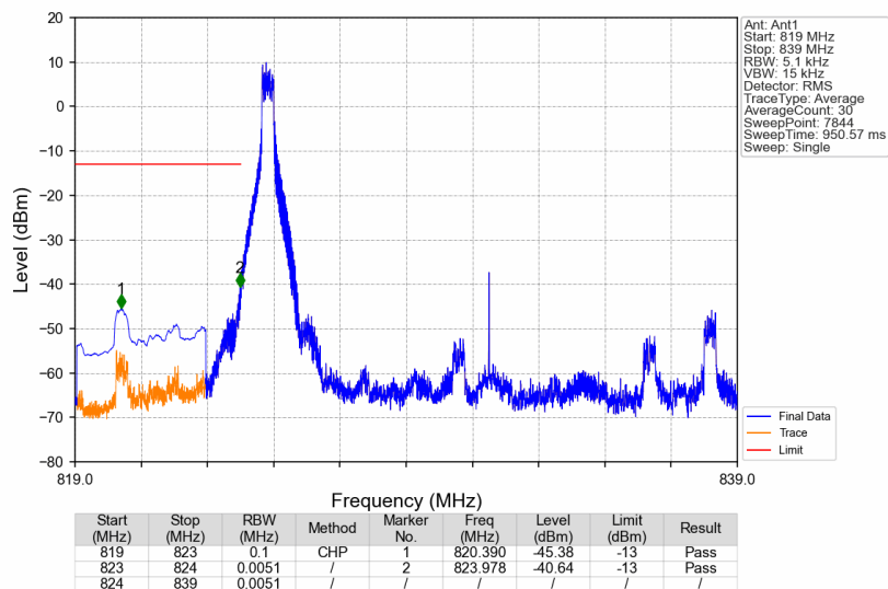
n5_30kHz_SISO_NTNV_15MHz_DFT-s-OFDM PI/2 BPSK 831.5MHz_Edge_1RB_Left
