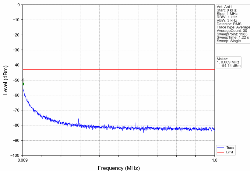
n7_15kHz_SISO_NTNV_5MHz_DFT-s-OFDM_PI/2_BPSK_2502.5MHz_Edge_1RB_Left
