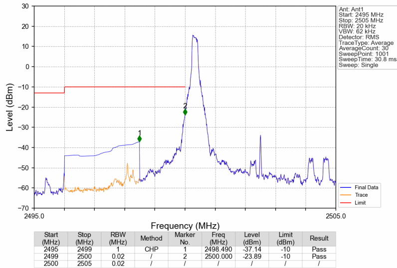
n7_15kHz_SISO_NTNV_5MHz_DFT-s-OFDM_PI/2_BPSK_2502.5MHz_Edge_1RB_Left
