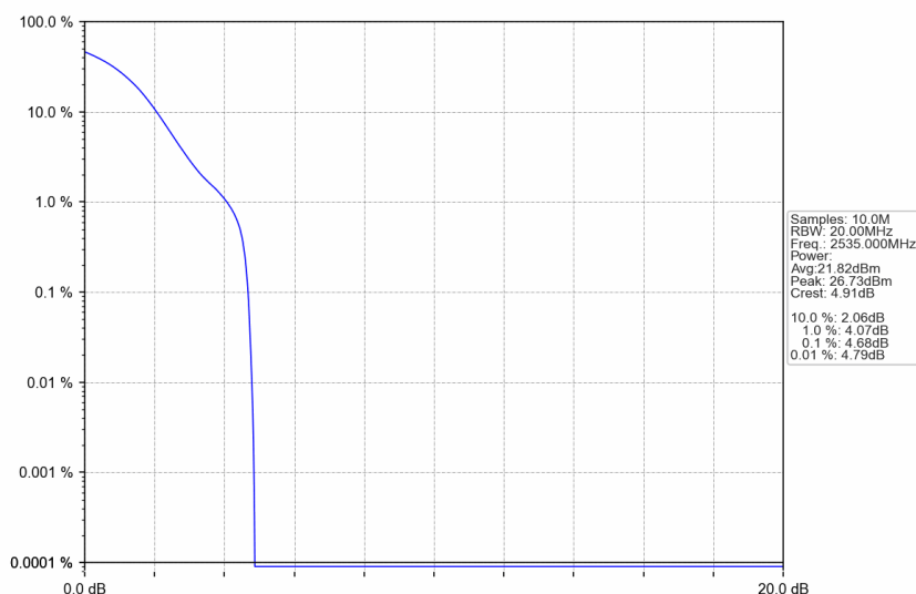
n7_15kHz_SISO_NTNV_25MHz_DFT-s-OFDM PI/2 BPSK_2535MHz_Outer_Full
