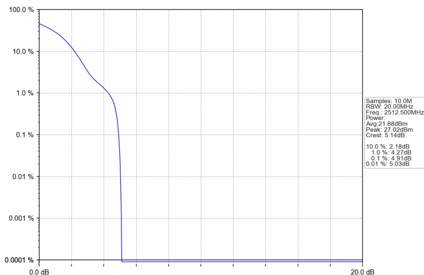
n7_15kHz_SISO_NTNV_25MHz_DFT-s-OFDM PI/2 BPSK_2512.5MHz_Outer_Full
