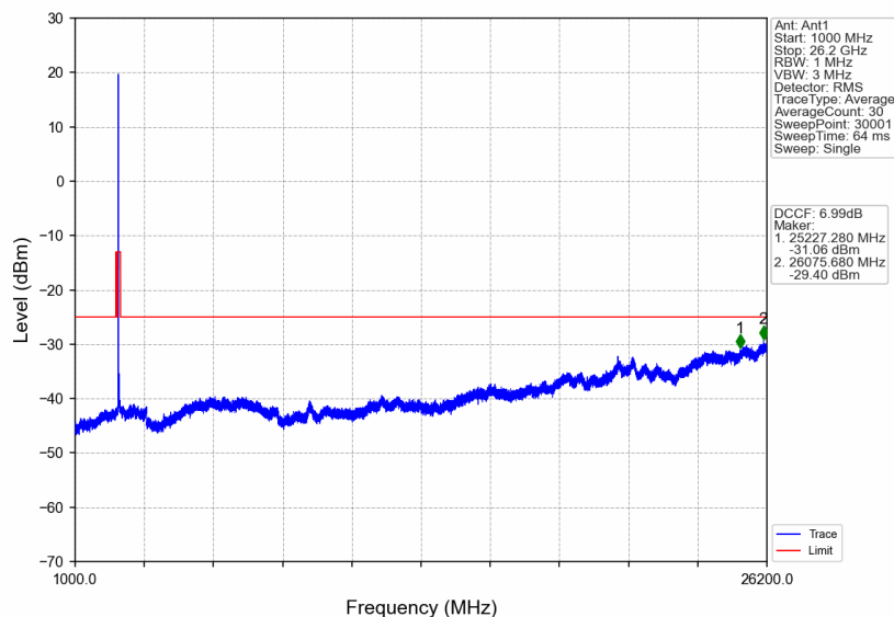
n38 30kHz SISO NTNV 30MHz DFT-s-OFDM PI/2 BPSK 2585MHz Outer Full
