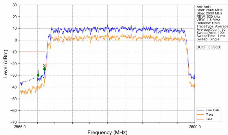
n38 30kHz SISO NTNV 30MHz DFT-s-OFDM PI/2 BPSK 2585MHz Outer Full
