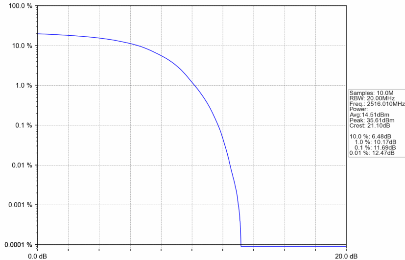
n41_15kHz_SISO_NTNV_40MHz_DFT-s-OFDM_PI/2_BPSK_2516.01MHz_Outer_Full
