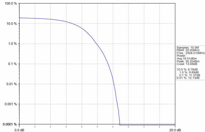
n41_30kHz_SISO_NTNV_25MHz_DFT-s-OFDM_PI/2_BPSK_2508.51MHz_Outer_Full
