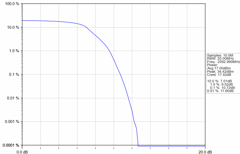
n41_30kHz_SISO_NTNV_20MHz_DFT-s-OFDM_PI/2_BPSK_2592.99MHz_Outer_Full
