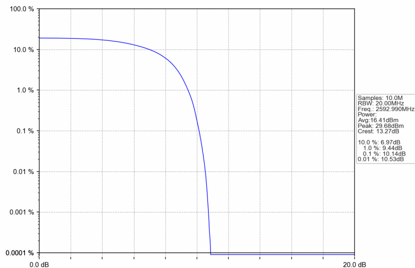
n41_30kHz_SISO_NTNV_25MHz_DFT-s-OFDM_PI/2_BPSK_2592.99MHz_Outer_Full
