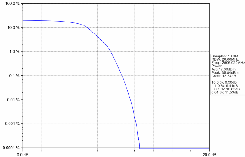
n41_30kHz_SISO_NTNV_20MHz_DFT-s-OFDM_PI/2_BPSK_2506.02MHz_Outer_Full
