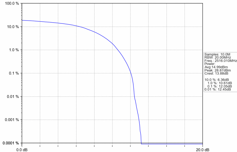
n41_30kHz_SISO_NTNV_40MHz_DFT-s-OFDM_PI/2_BPSK_2516.01MHz_Outer_Full
