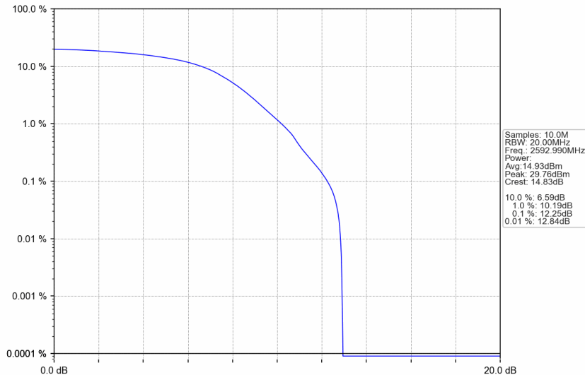
n41_30kHz_SISO_NTNV_40MHz_DFT-s-OFDM_PI/2_BPSK_2592.99MHz_Outer_Full
