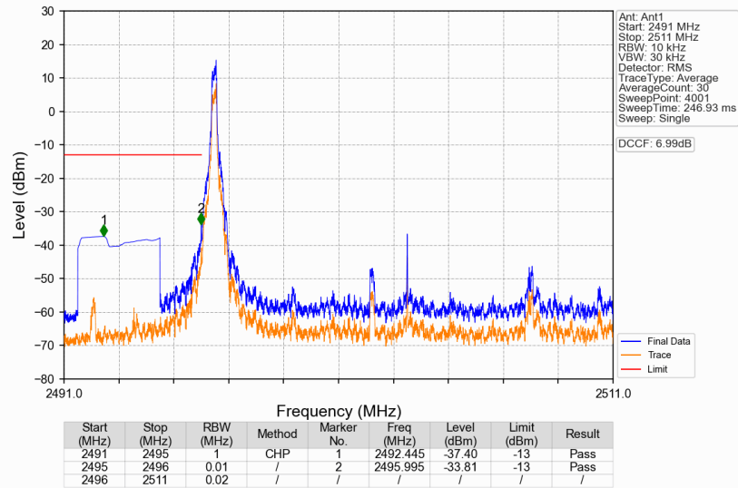
n41_15kHz_SISO_NTNV_15MHz_DFT-s-OFDM PI/2 BPSK_2503.5MHz_Edge_1RB_Left
