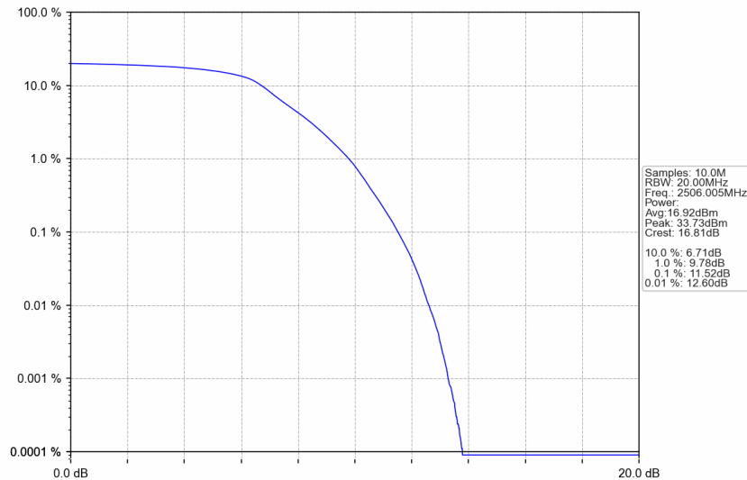
n41_15kHz_SISO_NTNV_20MHz_DFT-s-OFDM_PI/2_BPSK_2506.005MHz_Outer_Full
