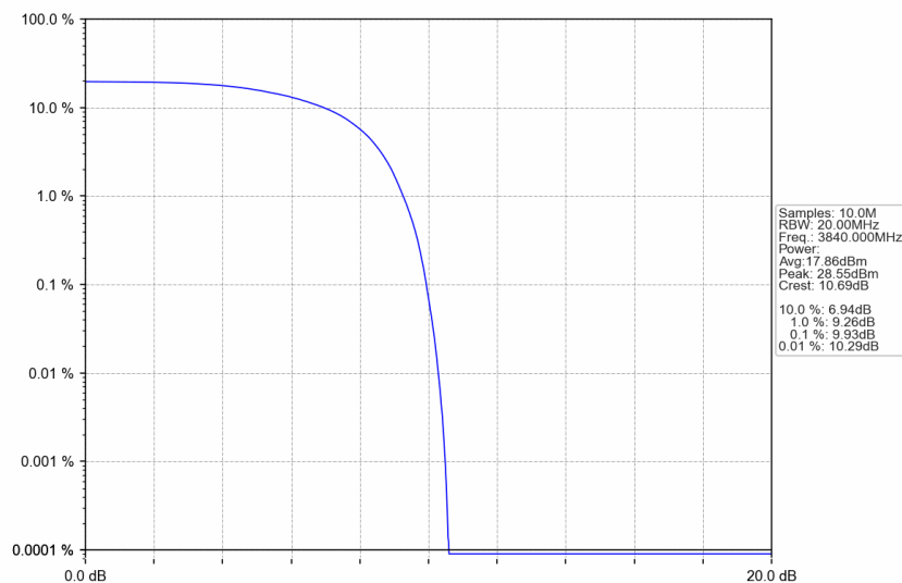
n77a_30kHz_SISO_NTNV_25MHz_DFT-s-OFDM PI/2 BPSK_3840MHz_Outer_Full
