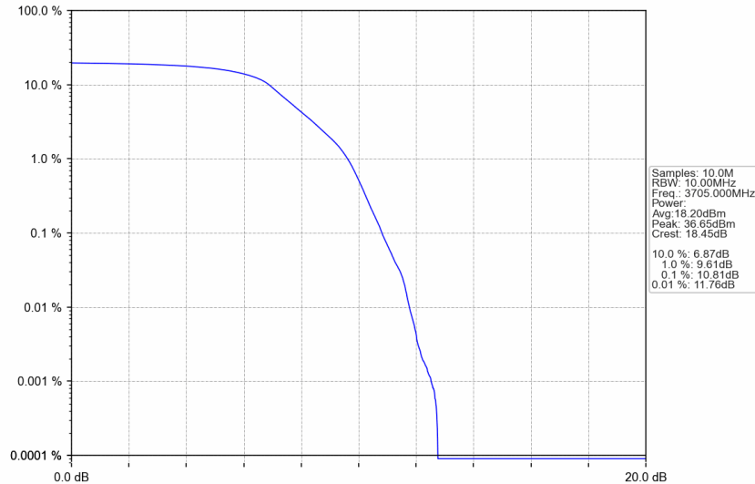
n77a_30kHz_SISO_NTNV_10MHz_DFT-s-OFDM PI/2 BPSK_3705MHz_Outer_Full
