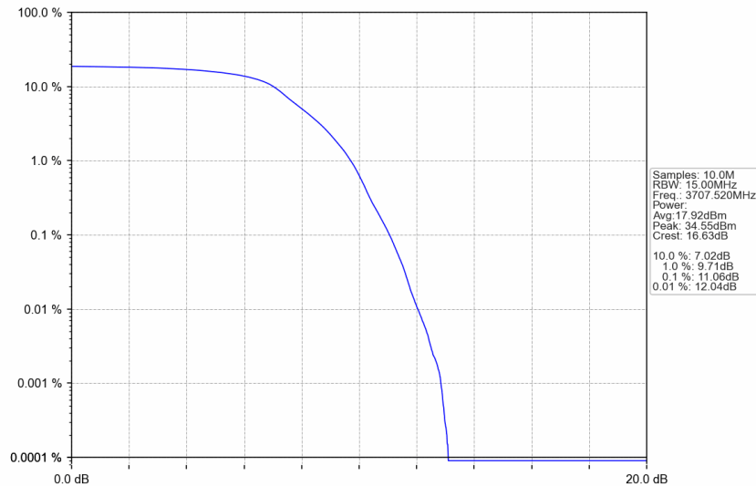
n77a_30kHz_SISO_NTNV_15MHz_DFT-s-OFDM PI/2 BPSK_3707.52MHz_Outer_Full
