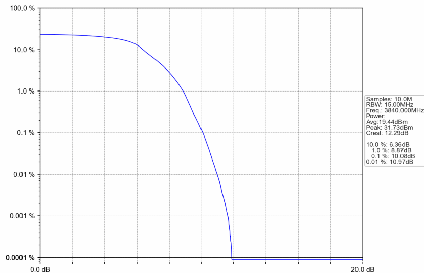
n77a_30kHz_SISO_NTNV_15MHz_DFT-s-OFDM PI/2 BPSK_3840MHz_Outer_Full
