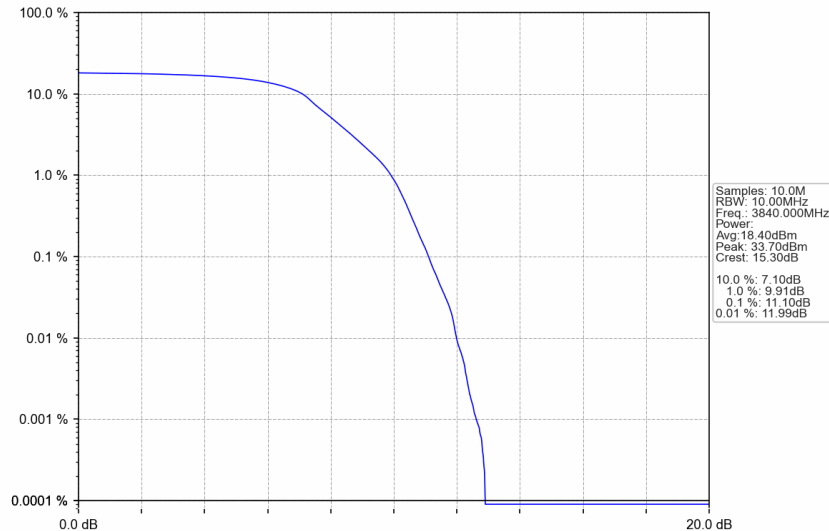
n77a_30kHz_SISO_NTNV_10MHz_DFT-s-OFDM PI/2 BPSK_3840MHz_Outer_Full
