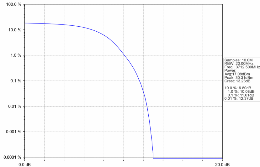
n77a_30kHz_SISO_NTNV_25MHz_DFT-s-OFDM PI/2 BPSK_3712.5MHz_Outer_Full
