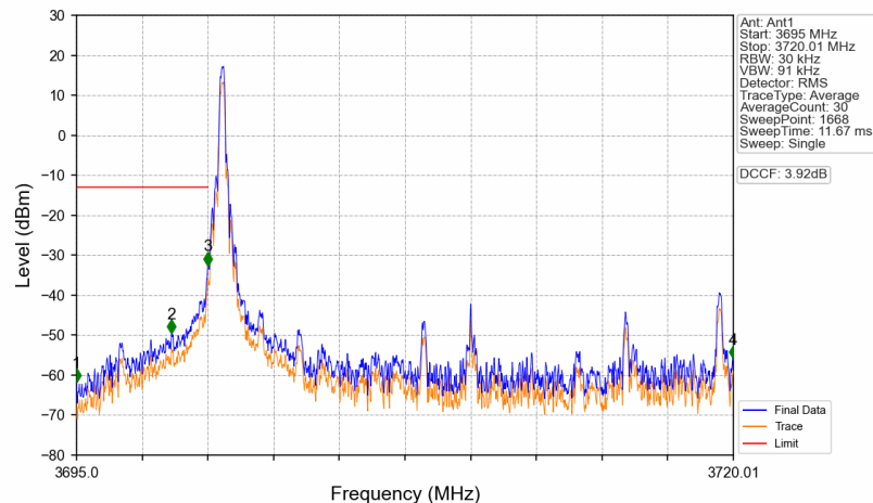
n77a_15kHz_SISO_NTNV_20MHz_DFT-s-OFDM PI/2 BPSK 3710.01MHz_Edge_1RB_Left
