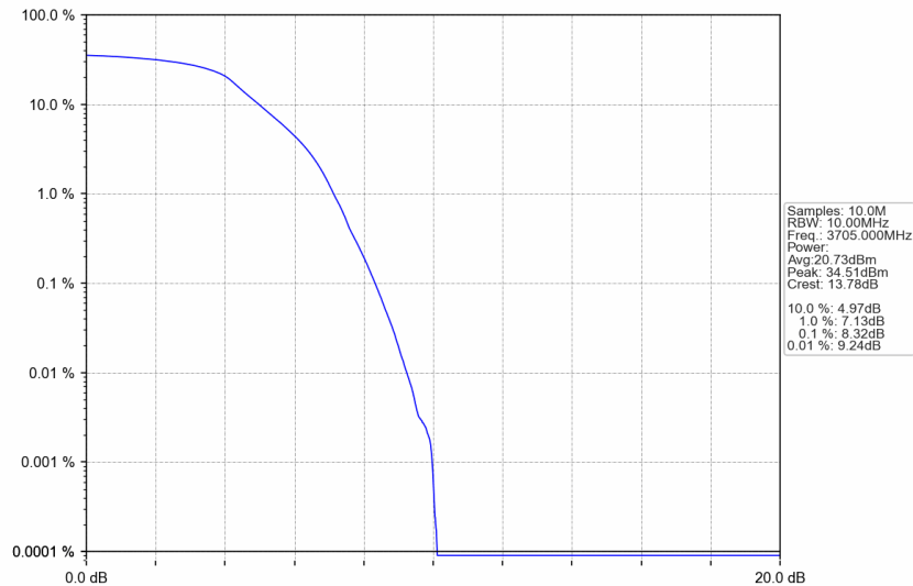
n77a_15kHz_SISO_NTNV_10MHz_DFT-s-OFDM PI/2 BPSK_3705MHz_Outer_Full
