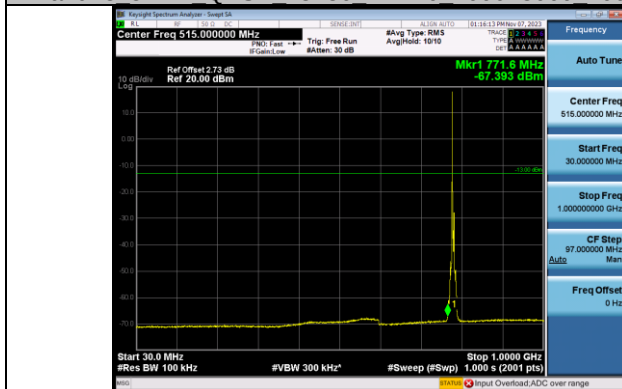
Band13 5MHz QPSK 23255 1RB#0 30~1000 30~1000
