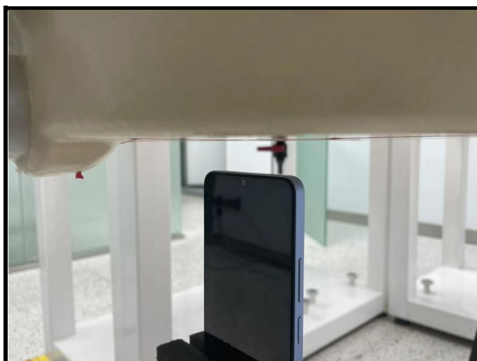
Top Side of EUT with 1.8 cm Gap
