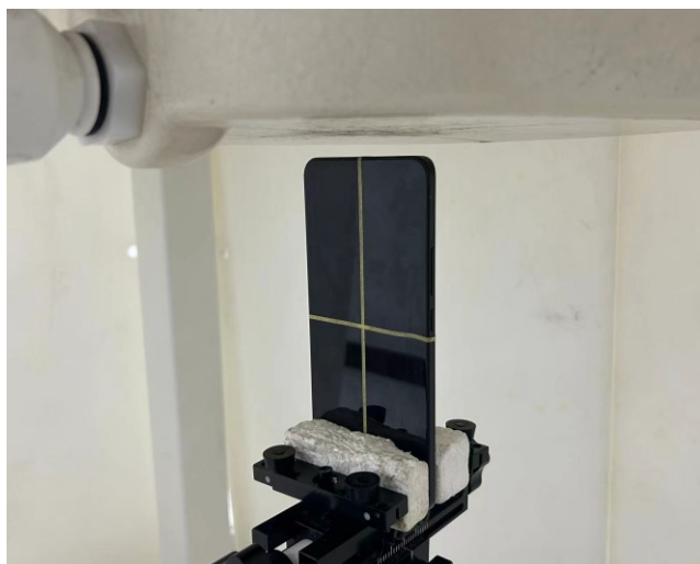
Top Side, Test Separation 10 mm
