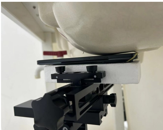
Left Cheek, Test Separation 0 mm
