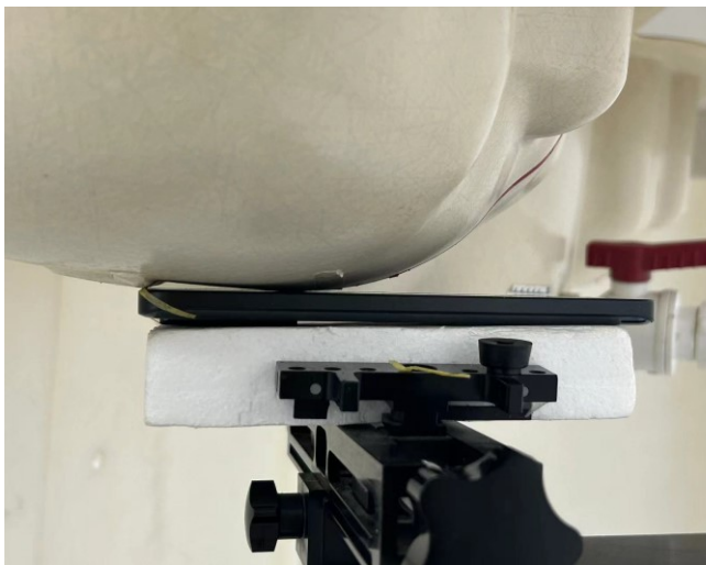
Right Cheek, Test Separation 0 mm
