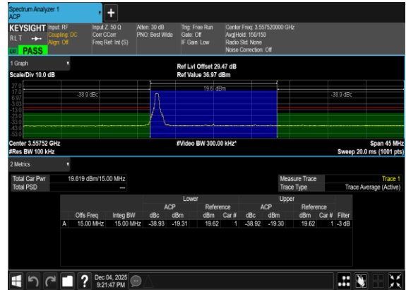
N48(15M)_DFT-s-OFDM_PI_2-BPSK_Edge_1RB_Left_Low_CH
