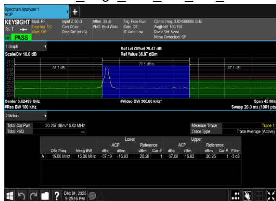
N48(15M)_DFT-s-OFDM_PI_2- BPSK_Edge_1RB_Left_Mid_CH
