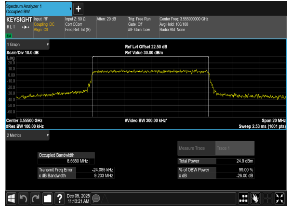
N48(10M)_CP-OFDM_16 QAM_Outer_Full_Low_CH
