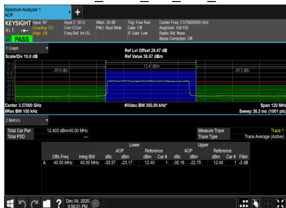
N48(40M)_DFT-s-OFDM_PI_2-BPSK_Outer_Full_Low_CH
