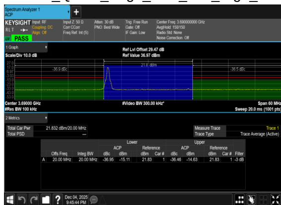
N48(20M)_DFT-s-OFDM_QPSK_Edge_1RB_Left_High_CH
