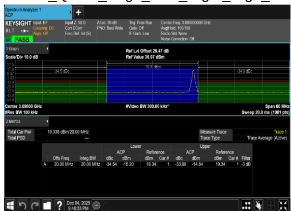
N48(20M)_DFT-s-OFDM_QPSK_Edge_1RB_Right_High_CH
