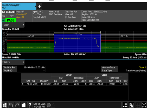
N48(15M)_DFT-s-OFDM_PI_2- BPSK_Outer_Full_Mid_CH
