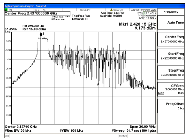
Mode:802.11be HE20 Tone:26T Frequency:2437MHz Ant:Chain0
