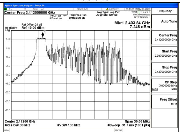
Mode:802.11be HE20 Tone:26T Frequency:2412MHz Ant:Chain1
