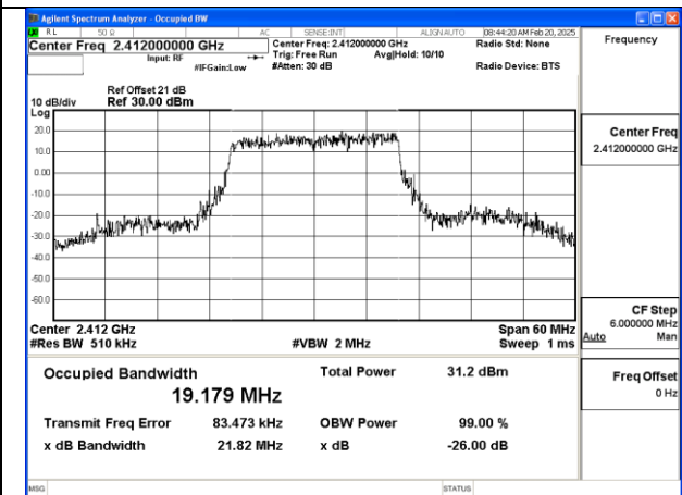
Mode:802.11be HE20 Tone:242T Frequency:2412MHz Ant:Chain1
