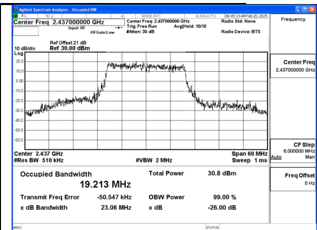
Mode:802.11be HE20 Tone:242T Frequency:2437MHz Ant:Chain0
