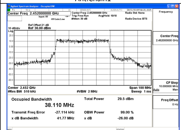
Mode:802.11be HE40 Tone:484T Frequency:2452MHz Ant:Chain1
