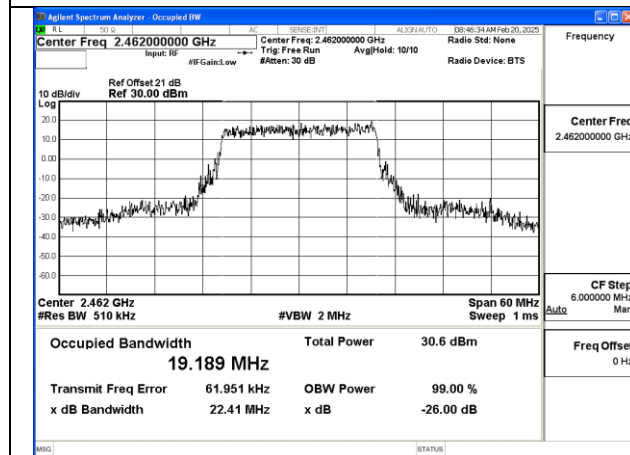
Mode:802.11be HE20 Tone:242T Frequency:2462MHz Ant:Chain0
