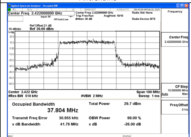
Mode:802.11be HE40 Tone:484T Frequency:2422MHz Ant:Chain1
