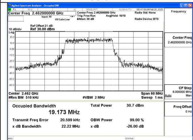
Mode:802.11be HE20 Tone:242T Frequency:2462MHz Ant:Chain1
