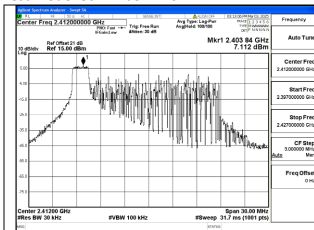
Mode:802.11be HE20 Tone:26T Frequency:2412MHz Ant:Chain0
