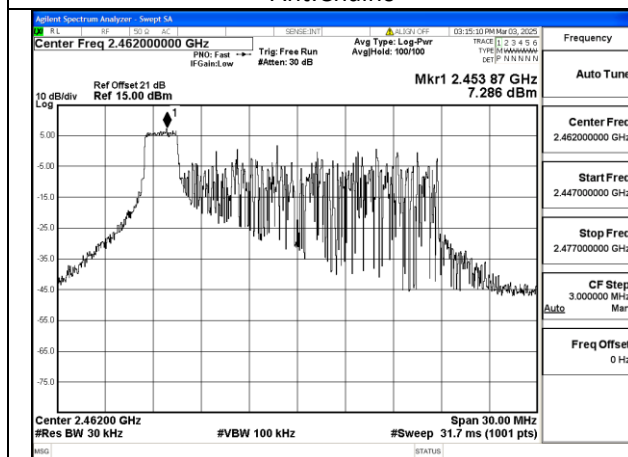
Mode:802.11be HE20 Tone:26T Frequency:2462MHz Ant:Chain0
