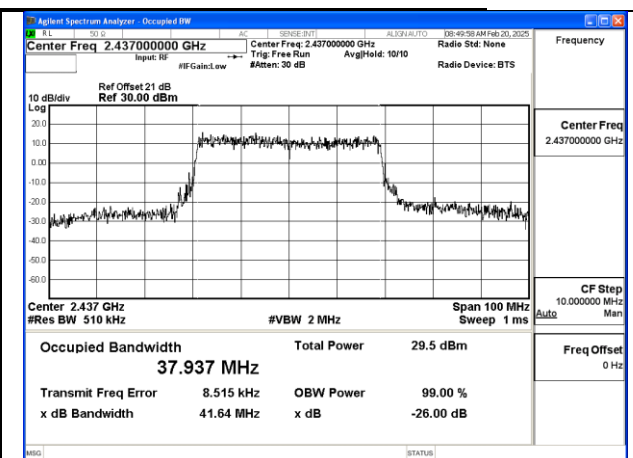
Mode:802.11be HE40 Tone:484T Frequency:2437MHz Ant:Chain0
