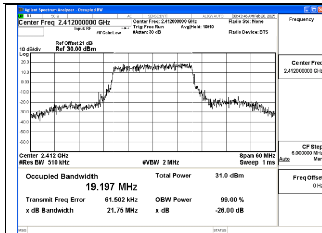
Mode:802.11be HE20 Tone:242T Frequency:2412MHz Ant:Chain0
