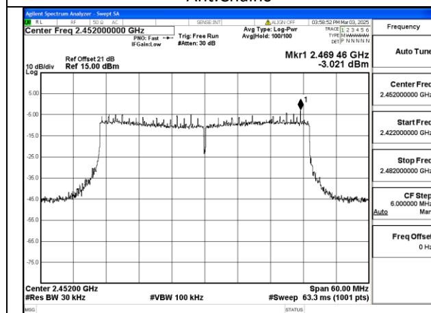
Mode:802.11be HE40 Tone:484T Frequency:2452MHz Ant:Chain0
