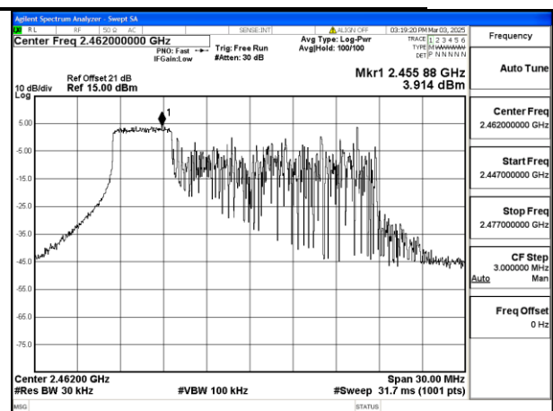
Mode:802.11be HE20 Tone:52T Frequency:2462MHz Ant:Chain1
