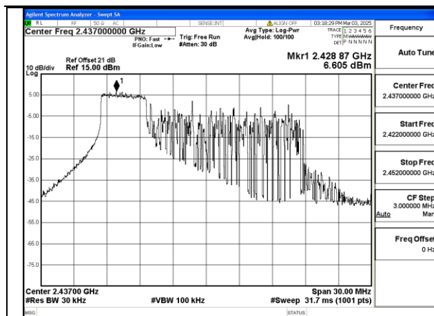
Mode:802.11be HE20 Tone:52T Frequency:2437MHz Ant:Chain1
