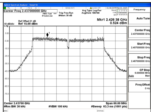
Mode:802.11n HT40 Frequency:2437MHz Ant:Chain0
