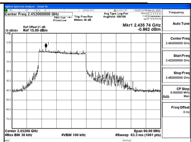
Mode:802.11be HE40 Tone:242T Frequency:2452MHz Ant:Chain1
