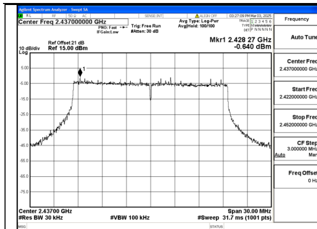
Mode:802.11be HE20 Tone:242T Frequency:2437MHz Ant:Chain1
