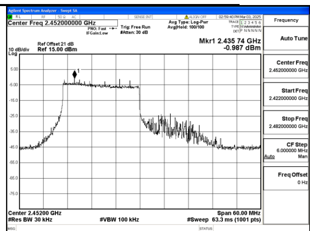
Mode:802.11ax HE40 Tone:242T Frequency:2452MHz Ant:Chain1
