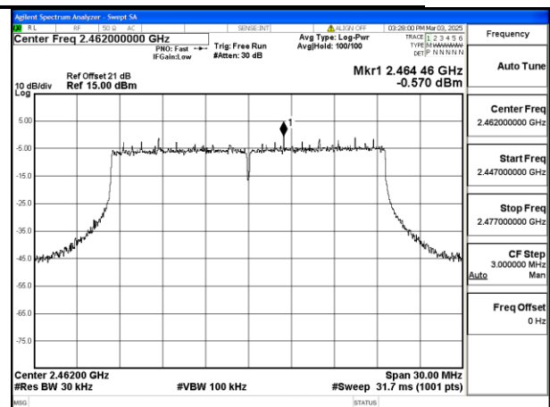
Mode:802.11be HE20 Tone:242T Frequency:2462MHz Ant:Chain1
