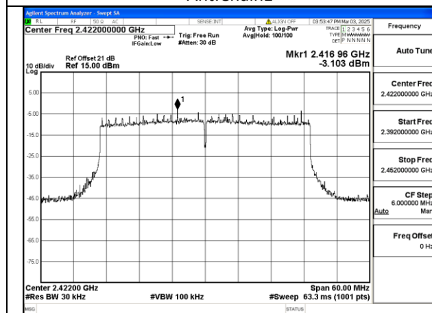
Mode:802.11be HE40 Tone:484T Frequency:2422MHz Ant:Chain0
