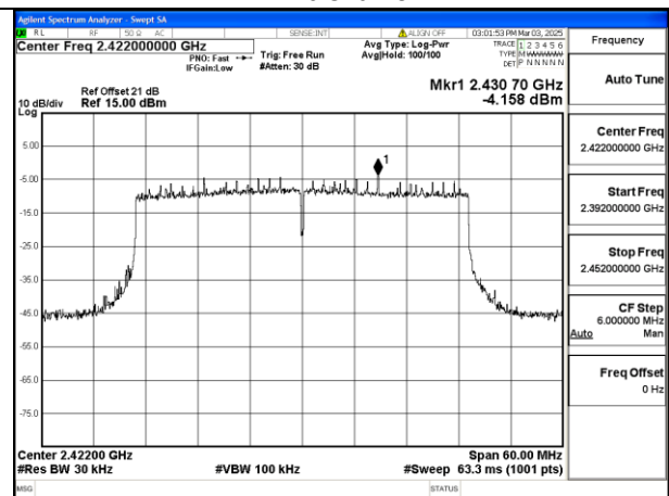
Mode:802.11ax HE40 Tone:484T Frequency:2422MHz Ant:Chain1
