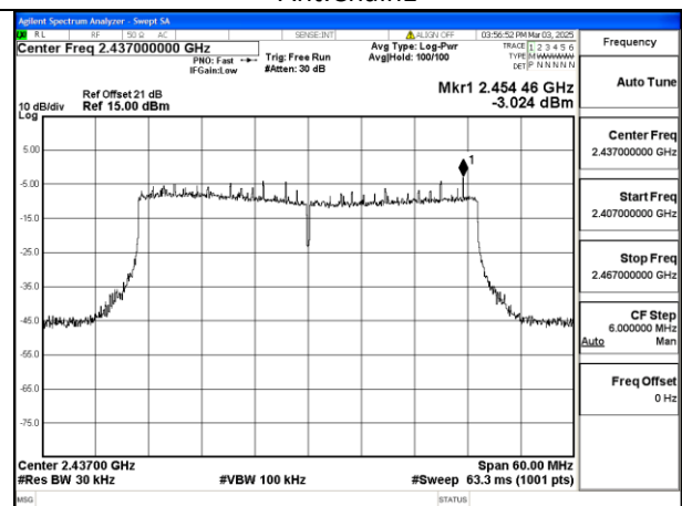
Mode:802.11be HE40 Tone:484T Frequency:2437MHz Ant:Chain0
