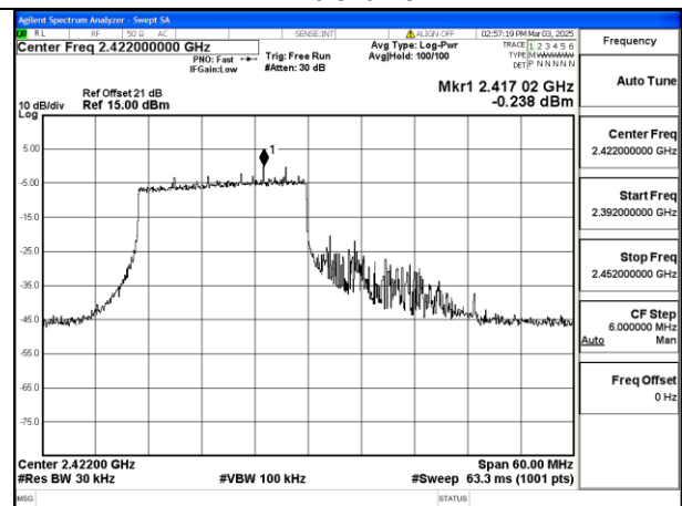
Mode:802.11ax HE40 Tone:242T Frequency:2422MHz Ant:Chain1
