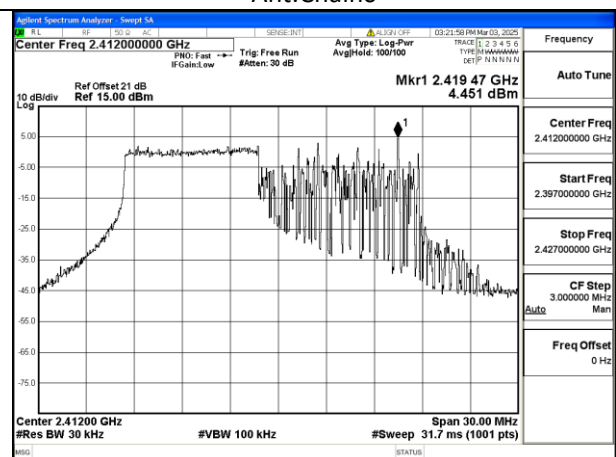
Mode:802.11be HE20 Tone:106T Frequency:2412MHz Ant:Chain1
