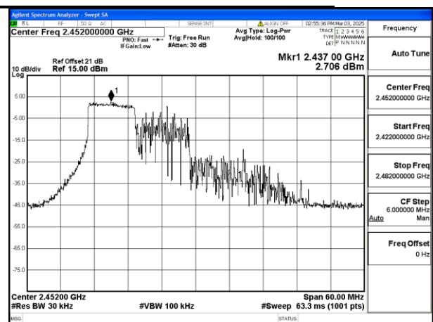
Mode:802.11ax HE40 Tone:106T Frequency:2452MHz Ant:Chain1
