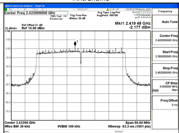
Mode:802.11be HE40 Tone:484T Frequency:2422MHz Ant:Chain1
