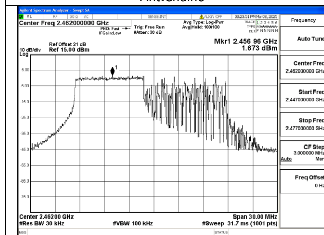
Mode:802.11be HE20 Tone:106T Frequency:2462MHz Ant:Chain0
