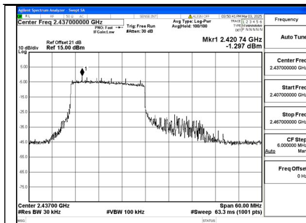
Mode:802.11be HE40 Tone:242T Frequency:2437MHz Ant:Chain1
