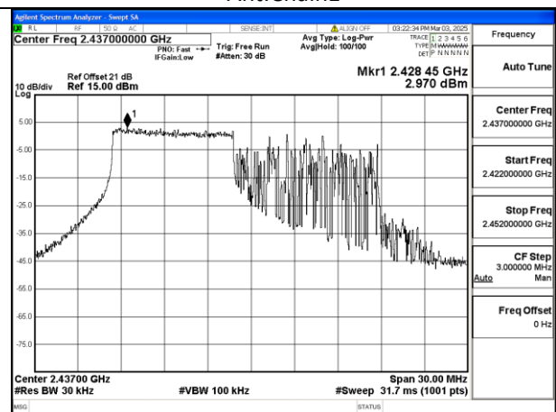
Mode:802.11be HE20 Tone:106T Frequency:2437MHz Ant:Chain0
