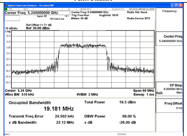
Mode:802.11be EHT20 Frequency:5240MHz Ant:Chain1
