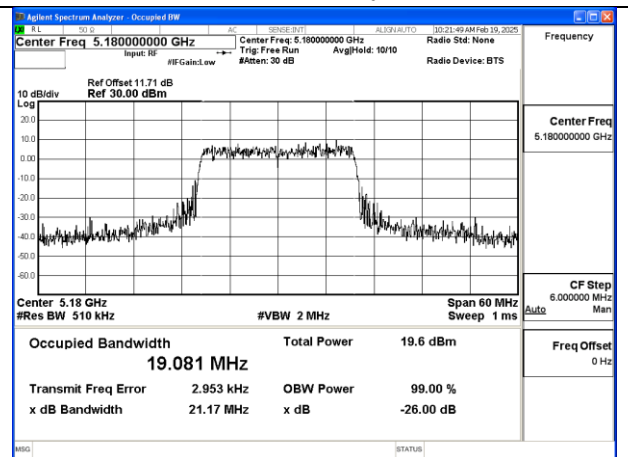
Mode:802.11be EHT20 Frequency:5180MHz Ant:Chain1
