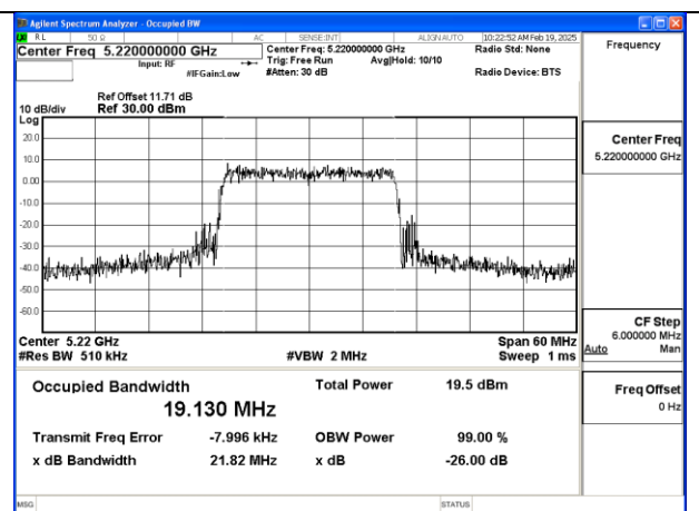
Mode:802.11be EHT20 Frequency:5220MHz Ant:Chain0
