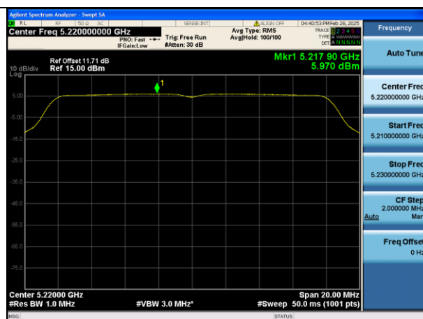
Mode:802.11a Frequency:5220MHz Ant:Chain0
