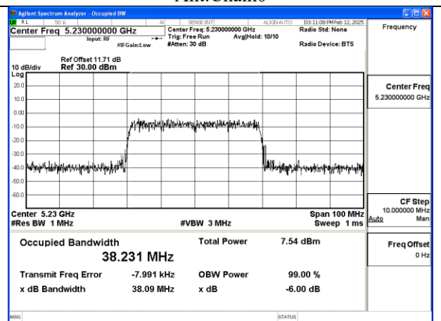
Mode:802.11ax HE40 Frequency:5230MHz Ant:Chain1
