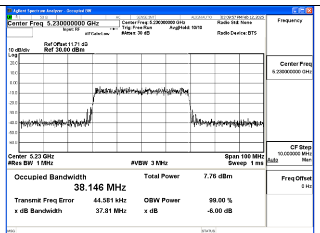
Mode:802.11ax HE40 Frequency:5230MHz Ant:Chain0
