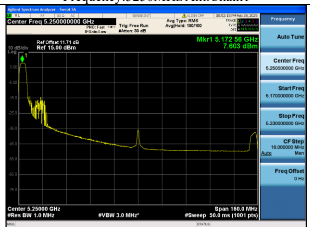
Mode:802.11ax HE160 Tone:52T Frequency:5250MHz Ant:Chain1
