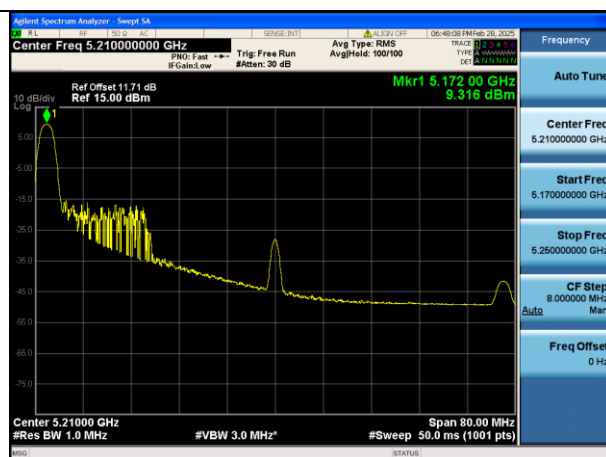
Mode:802.11be EHT80 Tone:26T Frequency:5210MHz Ant:Chain1
