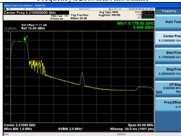
Mode:802.11be EHT80 Tone:106T Frequency:5210MHz Ant:Chain1
