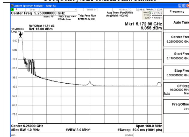
Mode:802.11be EHT160 Tone:52T Frequency:5250MHz Ant:Chain0
