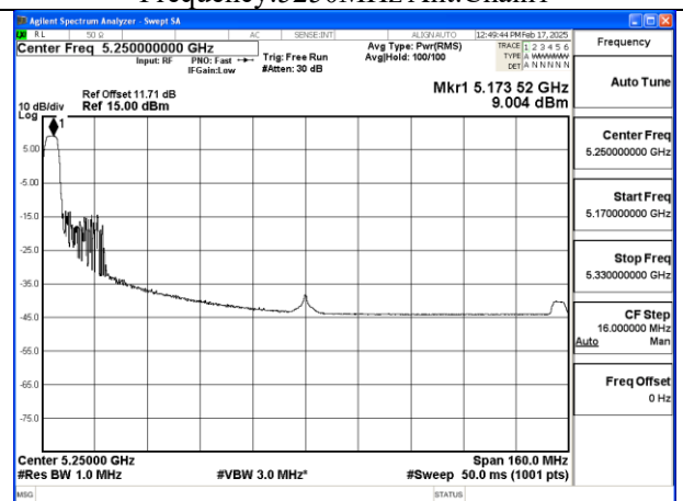
Mode:802.11be EHT160 Tone:52T Frequency:5250MHz Ant:Chain1
