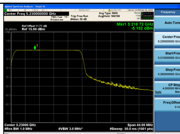
Mode:802.11be EHT40 Tone:242T Frequency:5230MHz Ant:Chain0
