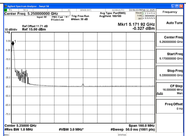
Mode:802.11ax HE160 Tone:26T Frequency:5250MHz Ant:Chain1
