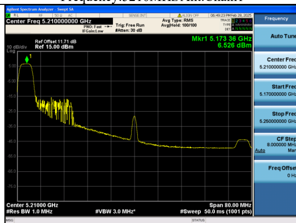
Mode:802.11be EHT80 Tone:52T Frequency:5210MHz Ant:Chain1
