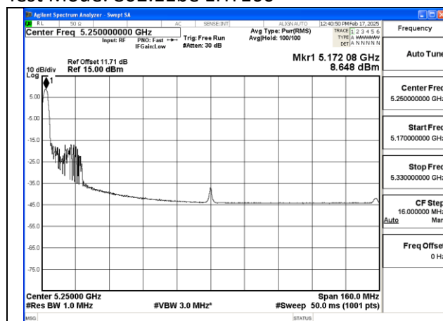
Mode:802.11be EHT160 Tone:26T Frequency:5250MHz Ant:Chain0
