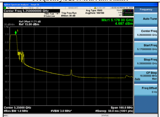
Mode:802.11ax HE160 Tone:106T Frequency:5250MHz Ant:Chain1
