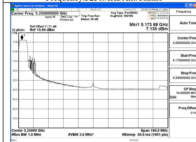
Mode:802.11be EHT160 Tone:106T Frequency:5250MHz Ant:Chain0
