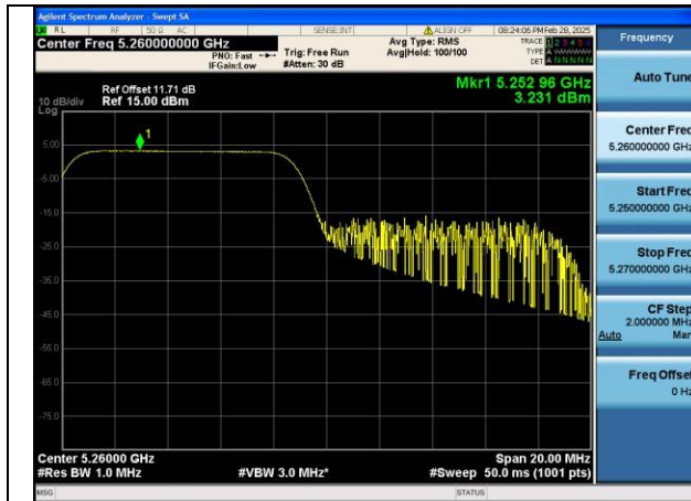
Mode:802.11be EHT20 Tone:106T Frequency:5260MHz Ant:Chain0
