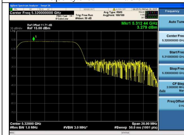
Mode:802.11be EHT20 Tone:106T Frequency:5320MHz Ant:Chain0
