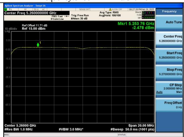
Mode:802.11be EHT20 Tone:242T Frequency:5260MHz Ant:Chain1
