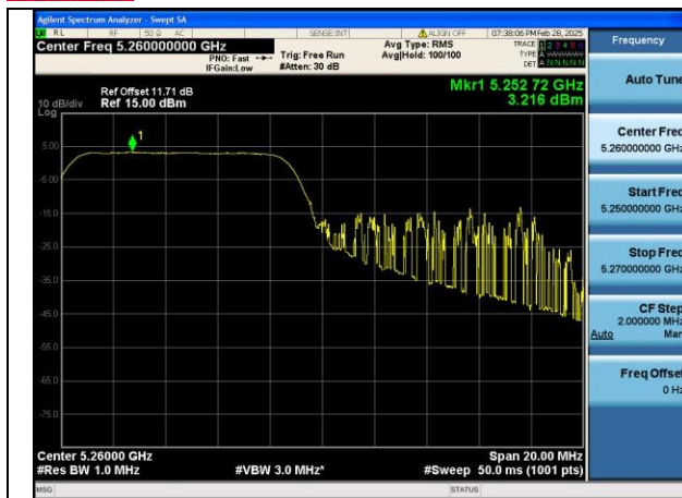
Mode:802.11ax HE20 Tone:106T Frequency:5260MHz Ant:Chain0
