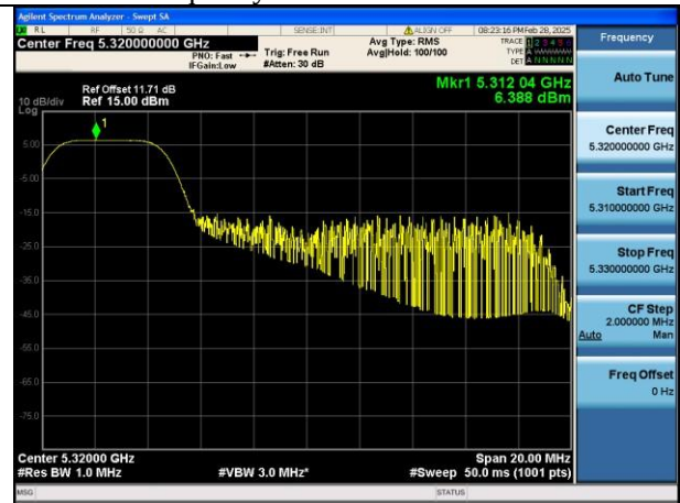
Mode:802.11be EHT20 Tone:52T Frequency:5320MHz Ant:Chain1
