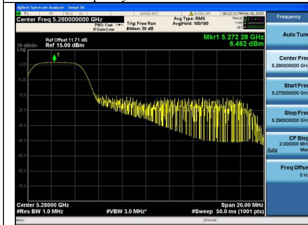
Mode:802.11be EHT20 Tone:52T Frequency:5280MHz Ant:Chain1
