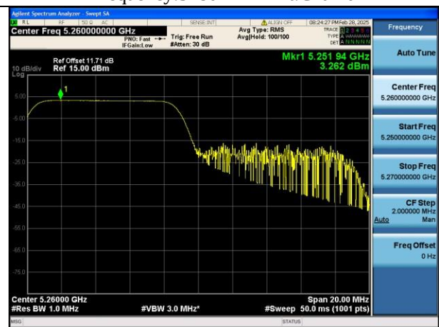
Mode:802.11be EHT20 Tone:106T Frequency:5260MHz Ant:Chain1
