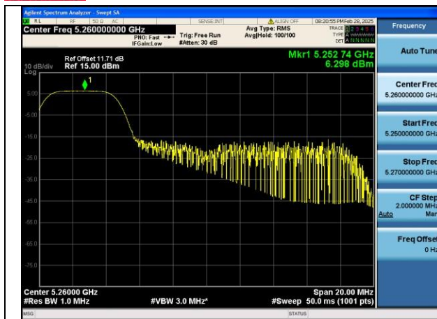
Mode:802.11be EHT20 Tone:52T Frequency:5260MHz Ant:Chain0
