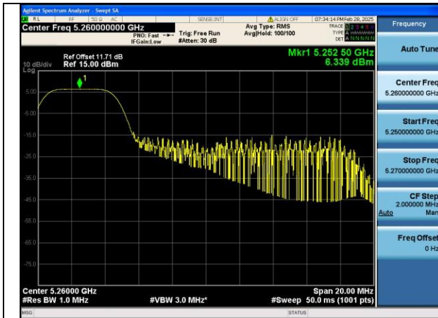
Mode:802.11ax HE20 Tone:52T Frequency:5260MHz Ant:Chain0
