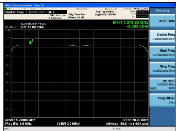
Mode:802.11ax HE20 Tone:242T Frequency:5280MHz Ant:Chain0
