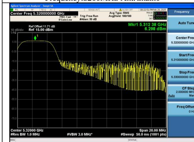
Mode:802.11be EHT20 Tone:52T Frequency:5320MHz Ant:Chain0
