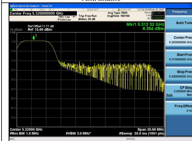
Mode:802.11ax HE20 Tone:52T Frequency:5320MHz Ant:Chain0
