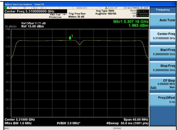
Mode:802.11ac VHT40 Frequency:5310MHz Ant:Chain0
