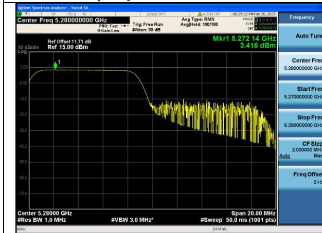
Mode:802.11be EHT20 Tone:106T Frequency:5280MHz Ant:Chain1
