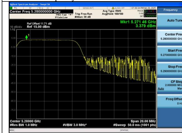
Mode:802.11ax HE20 Tone:106T Frequency:5280MHz Ant:Chain1
