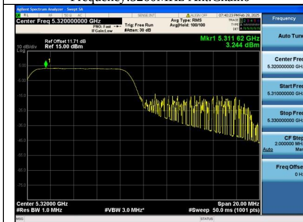
Mode:802.11ax HE20 Tone:106T Frequency:5320MHz Ant:Chain0
