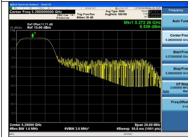
Mode:802.11ax HE20 Tone:52T Frequency:5280MHz Ant:Chain1
