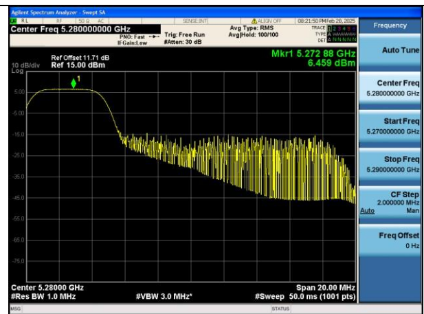
Mode:802.11be EHT20 Tone:52T Frequency:5280MHz Ant:Chain0
