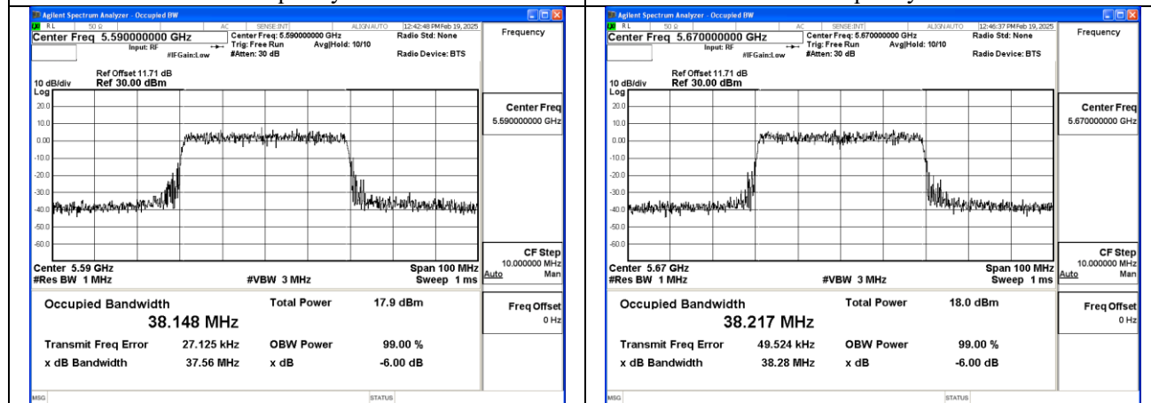
Mode:802.11n HT40 Frequency:5590MHz Ant:Chain1
