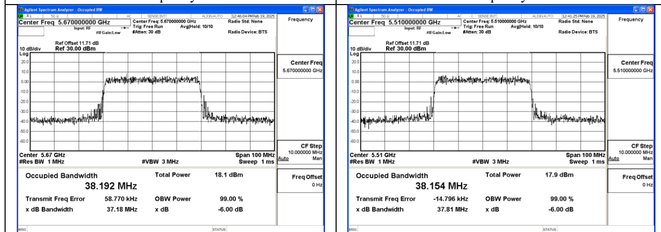
Mode:802.11n HT40 Frequency:5670MHz Ant:Chain0
