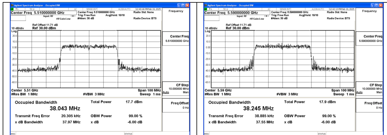
Mode:802.11n HT40 Frequency:5510MHz Ant:Chain0
