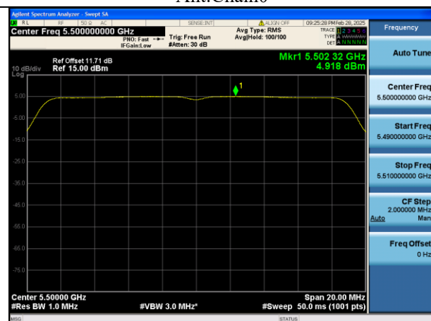
Mode:802.11ac VHT20 Frequency:5500MHz Ant:Chain1
