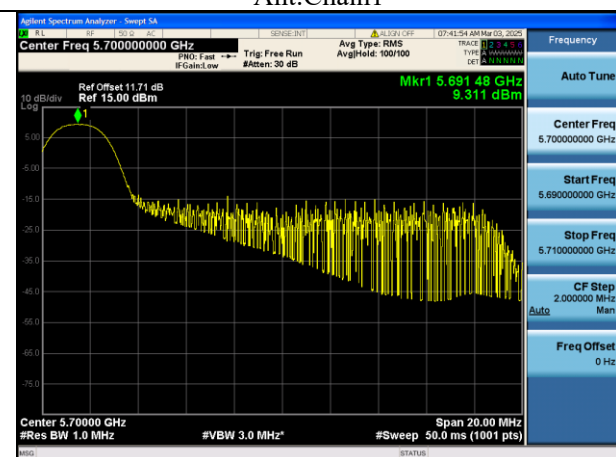
Mode:802.11ax HE20 Tone:26T Frequency:5700MHz Ant:Chain1
