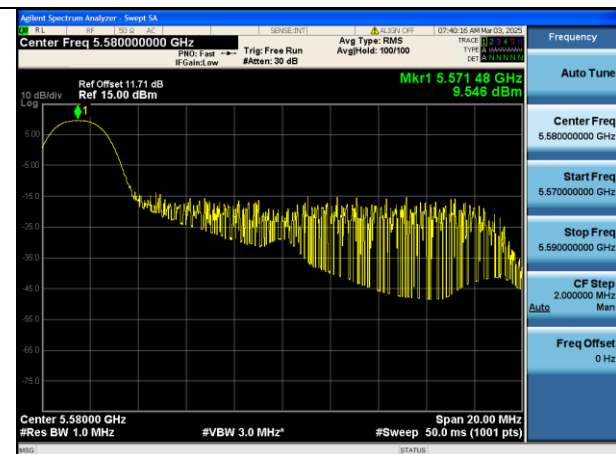
Mode:802.11ax HE20 Tone:26T Frequency:5580MHz Ant:Chain0
