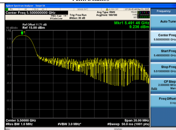
Mode:802.11ax HE20 Tone:26T Frequency:5500MHz Ant:Chain1
