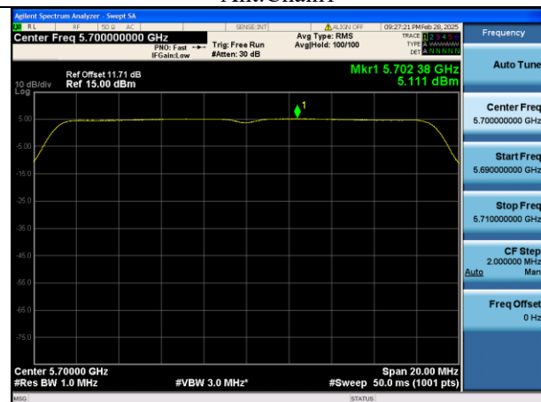
Mode:802.11ac VHT20 Frequency:5700MHz Ant:Chain1
