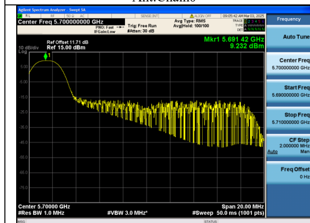
Mode:802.11be HE20 Tone:26T Frequency:5700MHz Ant:Chain0
