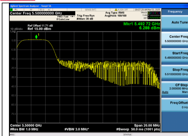
Mode:802.11be HE20 Tone:52T Frequency:5500MHz Ant:Chain0
