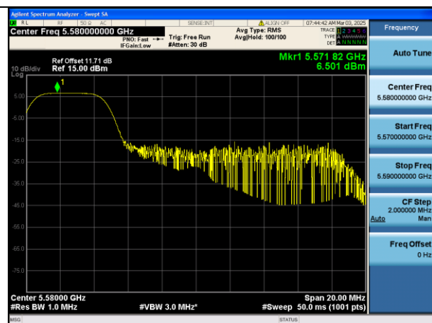
Mode:802.11ax HE20 Tone:52T Frequency:5580MHz Ant:Chain0
