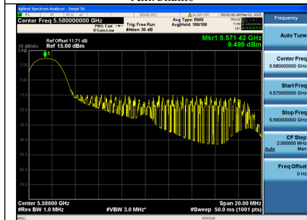
Mode:802.11be HE20 Tone:26T Frequency:5580MHz Ant:Chain1
