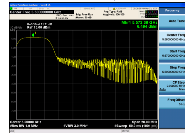
Mode:802.11be HE20 Tone:52T Frequency:5580MHz Ant:Chain1
