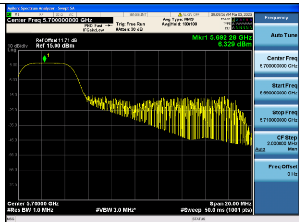
Mode:802.11be HE20 Tone:52T Frequency:5700MHz Ant:Chain1
