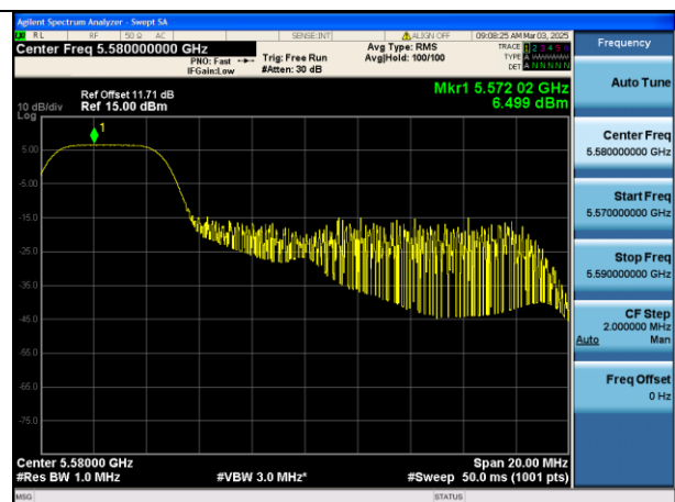
Mode:802.11be HE20 Tone:52T Frequency:5580MHz Ant:Chain0
