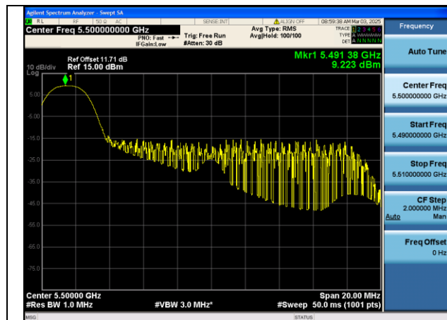
Mode:802.11be HE20 Tone:26T Frequency:5500MHz Ant:Chain0
