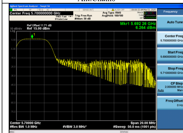
Mode:802.11be HE20 Tone:52T Frequency:5700MHz Ant:Chain0
