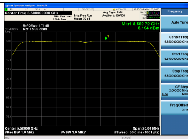
Mode:802.11ac VHT20 Frequency:5580MHz Ant:Chain0
