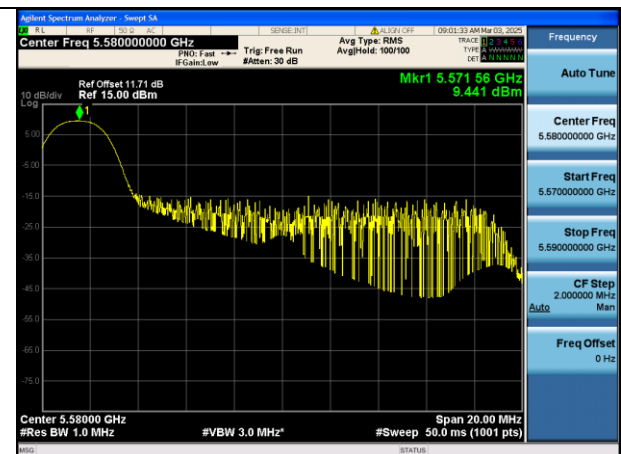
Mode:802.11be HE20 Tone:26T Frequency:5580MHz Ant:Chain0
