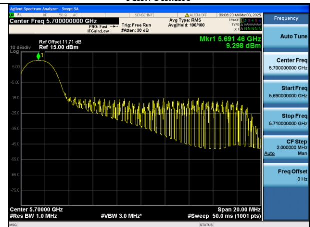
Mode:802.11be HE20 Tone:26T Frequency:5700MHz Ant:Chain1
