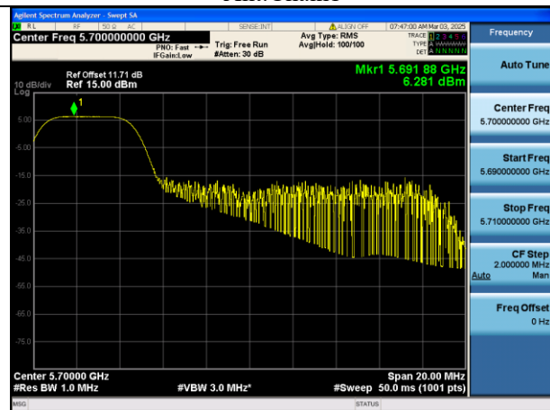
Mode:802.11ax HE20 Tone:52T Frequency:5700MHz Ant:Chain1
