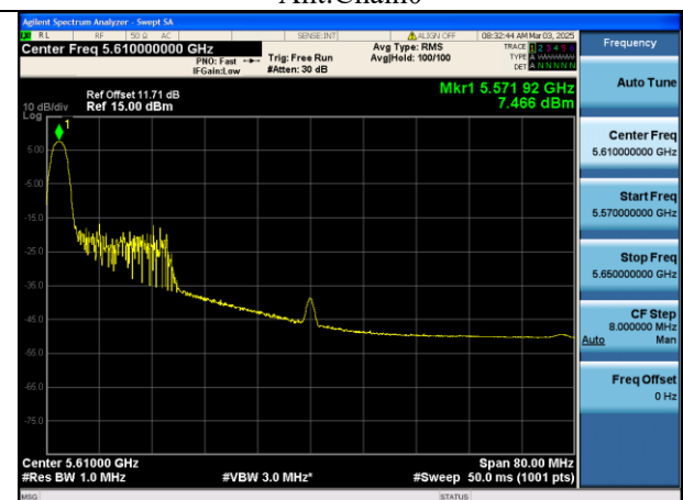
Mode:802.11ax HE80 Tone:26T Frequency:5610MHz Ant:Chain1
