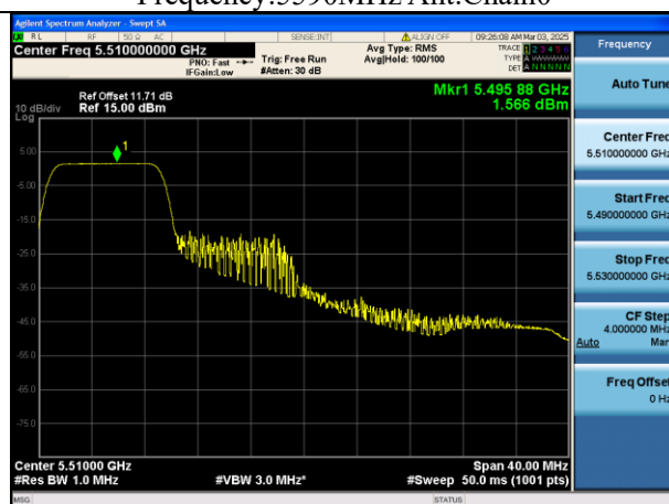
Mode:802.11be HE40 Tone:106T Frequency:5510MHz Ant:Chain1
