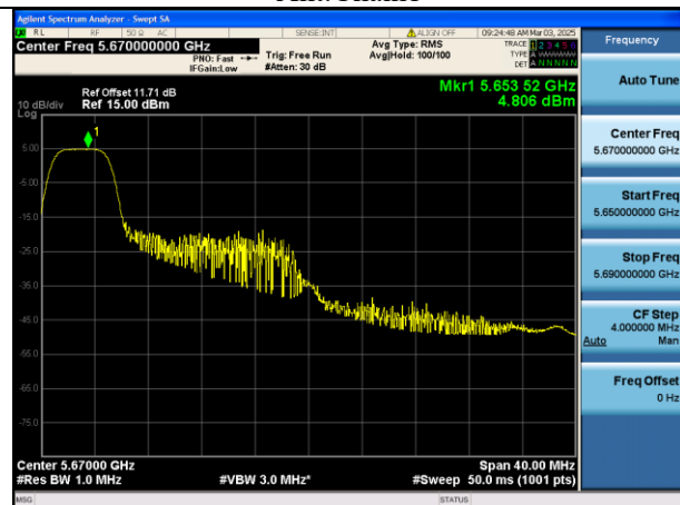
Mode:802.11be HE40 Tone:52T Frequency:5670MHz Ant:Chain1
