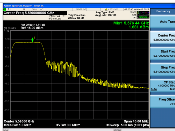
Mode:802.11be HE40 Tone:106T Frequency:5590MHz Ant:Chain0
