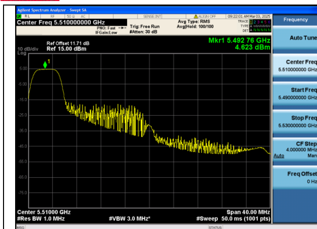
Mode:802.11be HE40 Tone:52T Frequency:5510MHz Ant:Chain0
