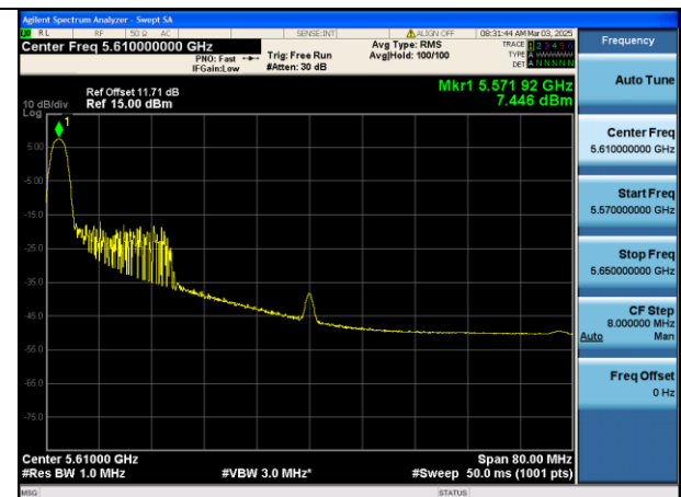
Mode:802.11ax HE80 Tone:26T Frequency:5610MHz Ant:Chain0
