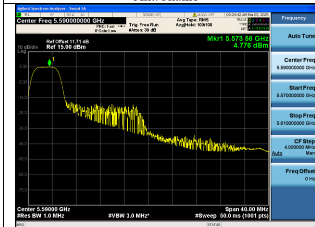
Mode:802.11be HE40 Tone:52T Frequency:5590MHz Ant:Chain1
