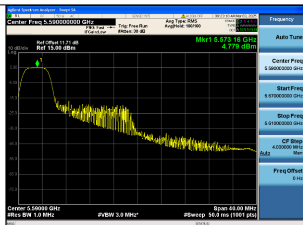
Mode:802.11be HE40 Tone:52T Frequency:5590MHz Ant:Chain0
