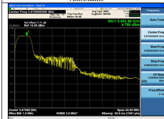
Mode:802.11be HE40 Tone:52T Frequency:5670MHz Ant:Chain0
