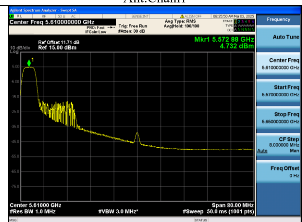
Mode:802.11ax HE80 Tone:52T Frequency:5610MHz Ant:Chain0
