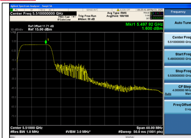
Mode:802.11be HE40 Tone:106T Frequency:5510MHz Ant:Chain0
