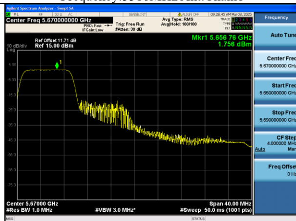
Mode:802.11be HE40 Tone:106T Frequency:5670MHz Ant:Chain1
