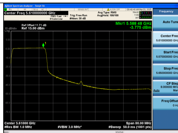
Mode:802.11be HE80 Tone:242T Frequency:5610MHz Ant:Chain0
