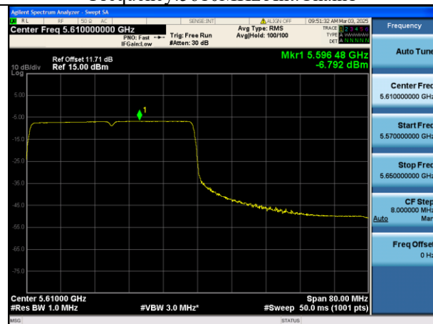
Mode:802.11be HE80 Tone:484T Frequency:5610MHz Ant:Chain0
