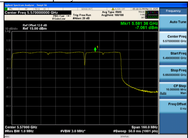
Mode:802.11be HE160 Tone:242+484+996 Frequency:5570MHz Ant:Chain1
