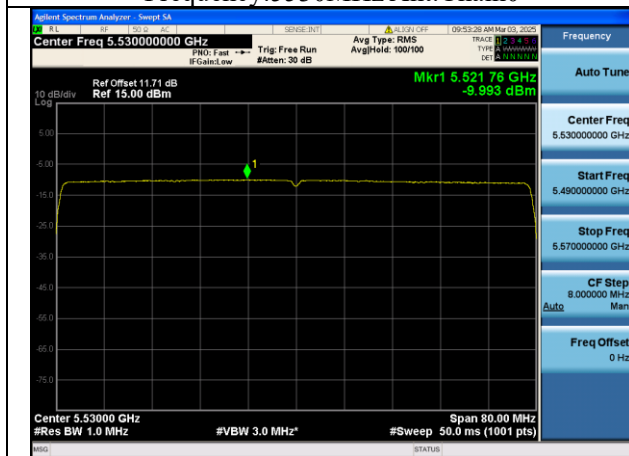
Mode:802.11be HE80 Tone:996T Frequency:5530MHz Ant:Chain1
