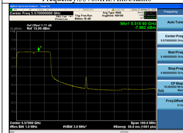
Mode:802.11be HE160 Tone:484T Frequency:5570MHz Ant:Chain0
