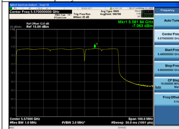
Mode:802.11be HE160 Tone:242+484+996 Frequency:5570MHz Ant:Chain0
