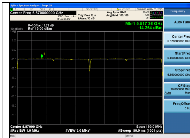
Mode:802.11be HE160 Tone:1992T Frequency:5570MHz Ant:Chain0
