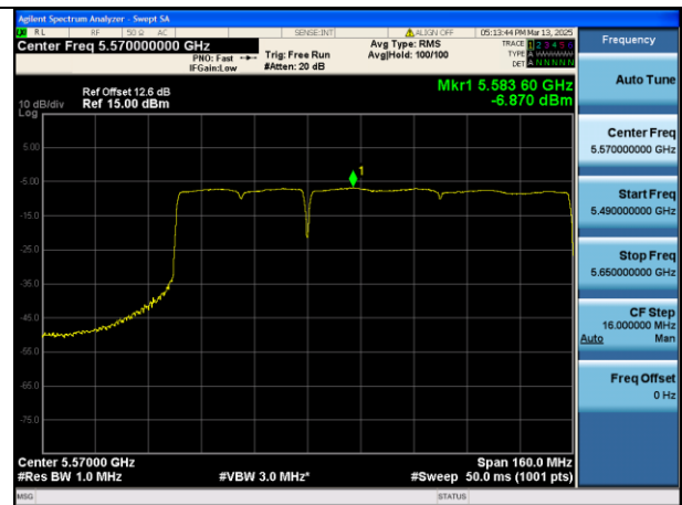
Mode:802.11be HE160 Tone:484+996 Frequency:5570MHz Ant:Chain1
