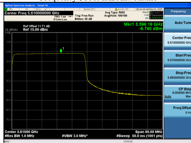
Mode:802.11ax HE80 Tone:484T Frequency:5610MHz Ant:Chain0
