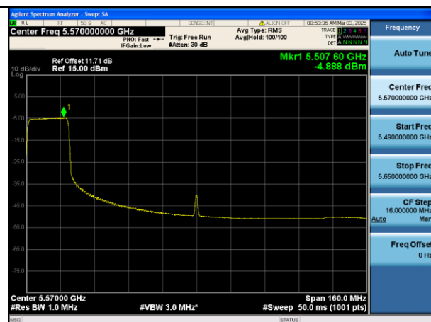
Mode:802.11ax HE160 Tone:242T Frequency:5570MHz Ant:Chain1
