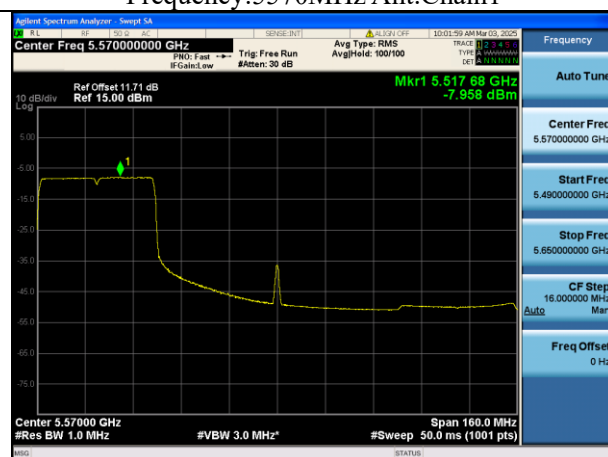
Mode:802.11be HE160 Tone:484T Frequency:5570MHz Ant:Chain1
