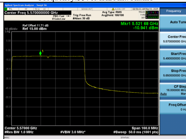
Mode:802.11ax HE160 Tone:996T Frequency:5570MHz Ant:Chain1
