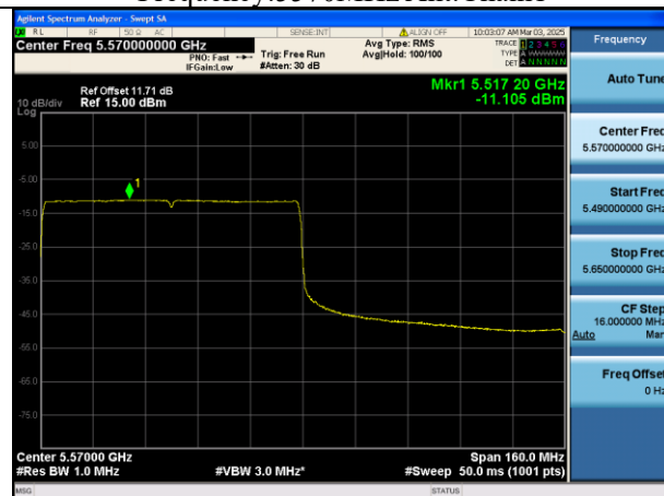
Mode:802.11be HE160 Tone:996T Frequency:5570MHz Ant:Chain1
