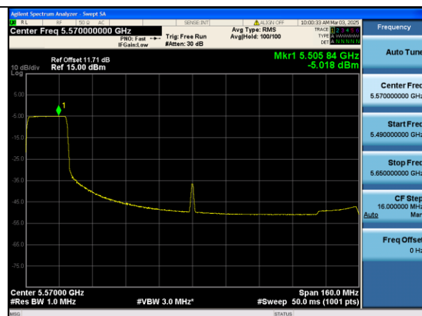
Mode:802.11be HE160 Tone:242T Frequency:5570MHz Ant:Chain1
