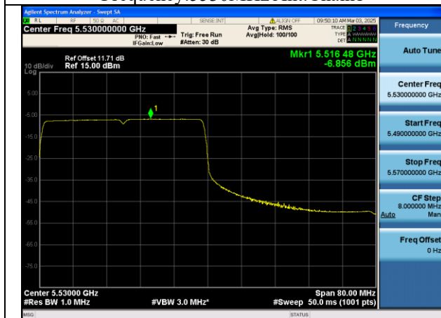
Mode:802.11be HE80 Tone:484T Frequency:5530MHz Ant:Chain0
