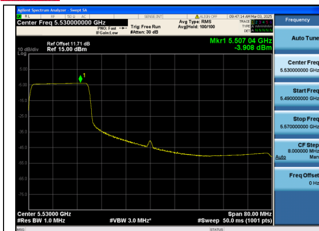
Mode:802.11be HE80 Tone:242T Frequency:5530MHz Ant:Chain0
