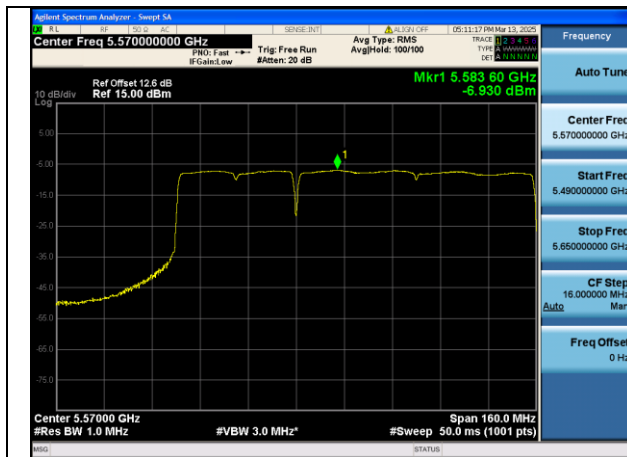
Mode:802.11be HE160 Tone:484+996 Frequency:5570MHz Ant:Chain0
