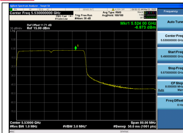
Mode:802.11be HE80 Tone:484T Frequency:5530MHz Ant:Chain1
