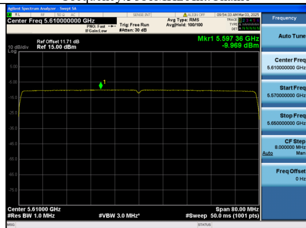
Mode:802.11be HE80 Tone:996T Frequency:5610MHz Ant:Chain1
