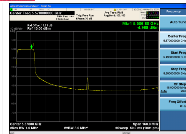
Mode:802.11be HE160 Tone:242T Frequency:5570MHz Ant:Chain0
