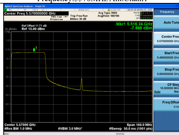
Mode:802.11ax HE160 Tone:484T Frequency:5570MHz Ant:Chain1
