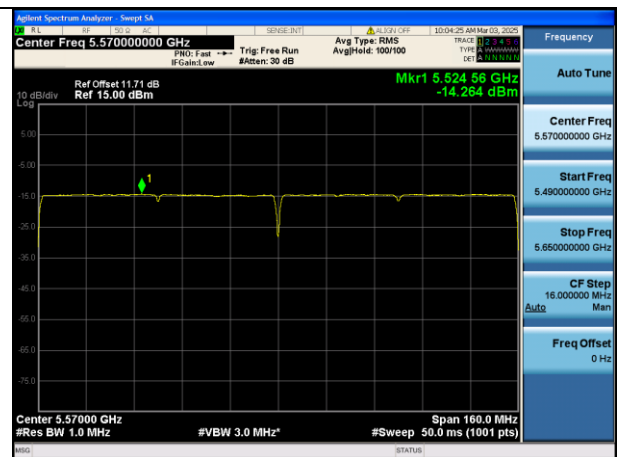
Mode:802.11be HE160 Tone:1992T Frequency:5570MHz Ant:Chain1
