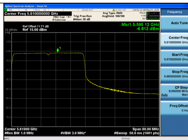
Mode:802.11be HE80 Tone:484T Frequency:5610MHz Ant:Chain1
