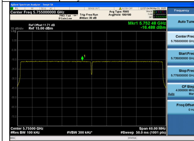
Mode:802.11be HE40 Tone:484T Frequency:5755MHz Ant:Chain0
