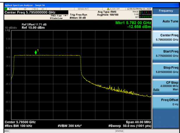
Mode:802.11be HE40 Tone:242T Frequency:5795MHz Ant:Chain0
