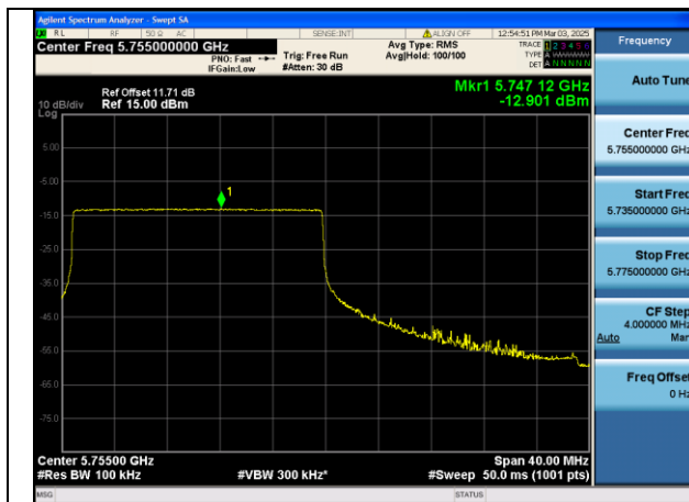
Mode:802.11be HE40 Tone:242T Frequency:5755MHz Ant:Chain0
