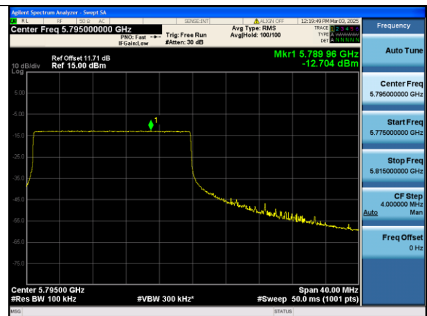
Mode:802.11ax HE40 Tone:242T Frequency:5795MHz Ant:Chain0
