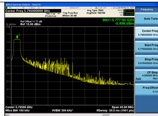
Mode:802.11ax HE40 Tone:26T Frequency:5795MHz Ant:Chain0
