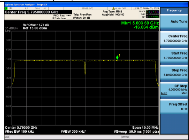
Mode:802.11be HE40 Tone:484T Frequency:5795MHz Ant:Chain0
