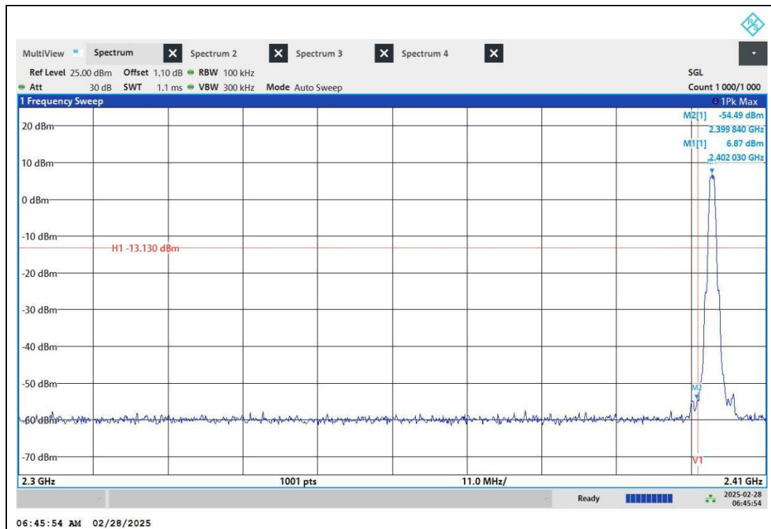
BLE_1M_ANT1_Low_2402
