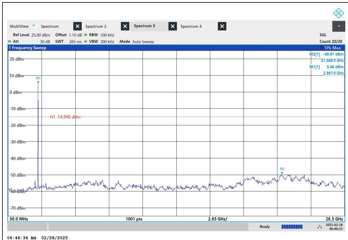
BLE_1M_ANT1_2402_30~26500
