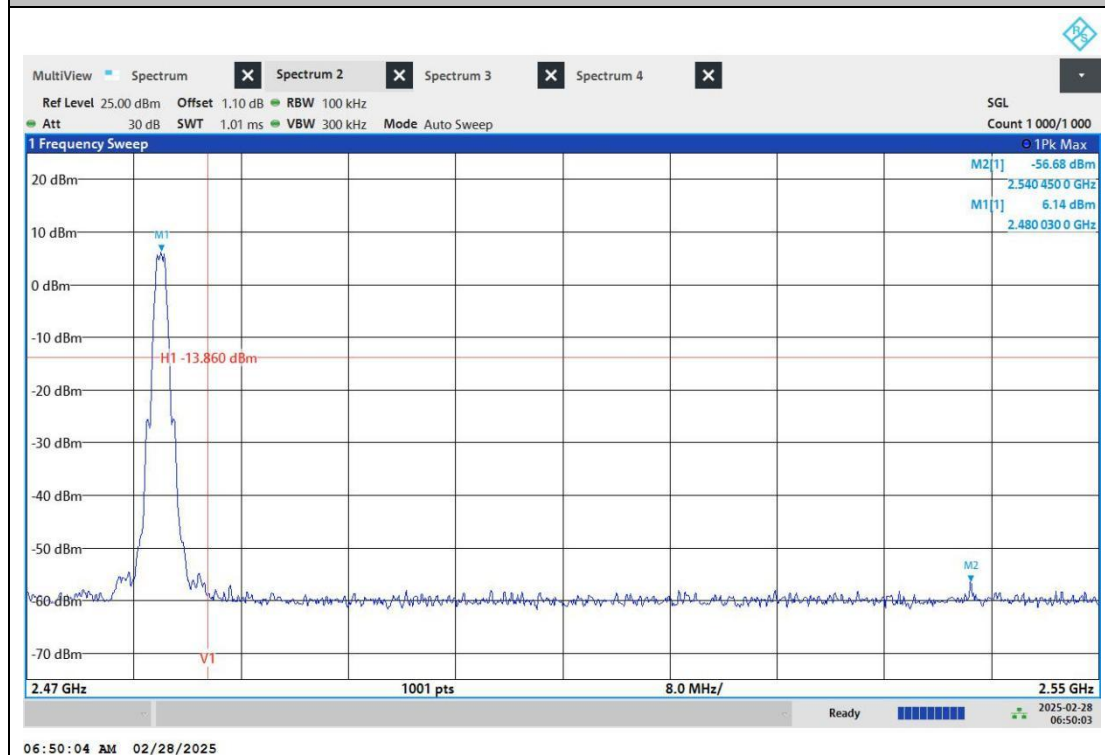
BLE_1M_ANT1_High_2480
