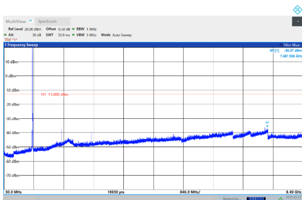
Band26-15MHz-QPSK-26865-1RB#0-Range:30~8490MHz
