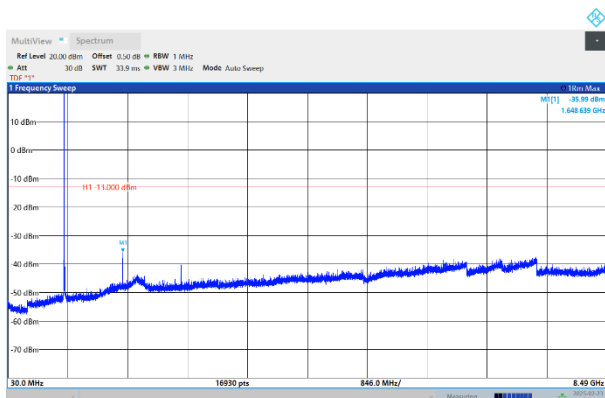
Band26-5MHz-QPSK-27015-1RB#0-Range:30~8490MHz
