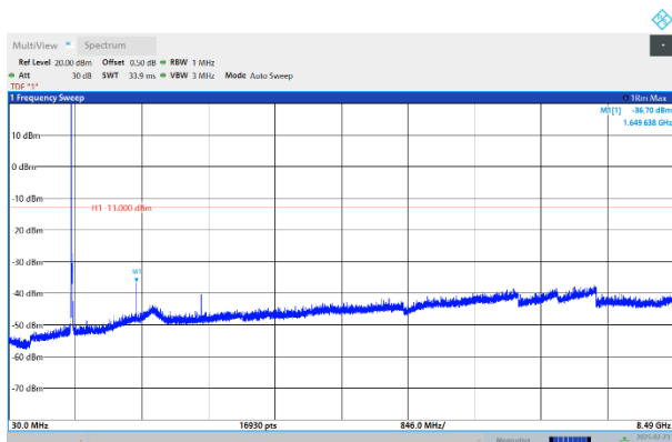
Band26-15MHz-QPSK-26965-1RB#0-Range:30~8490MHz
