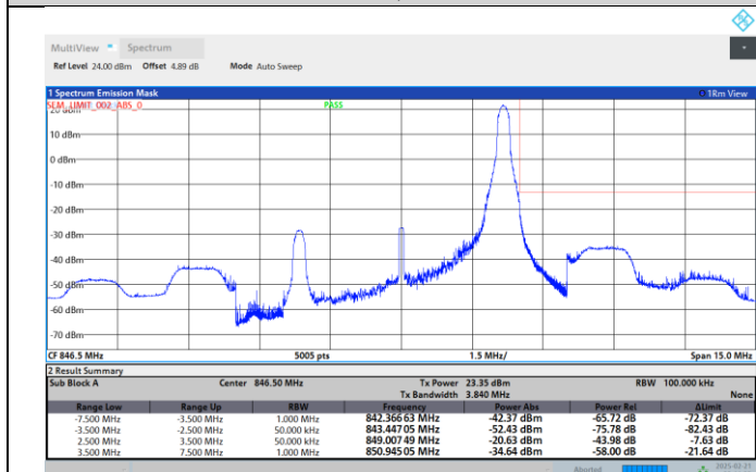
Band26-5MHz-64QAM-26815-1RB#0
