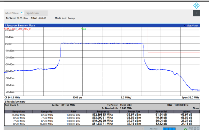
Band26-15MHz-256QAM-26865-75RB#0
