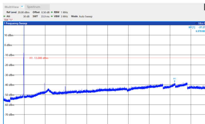
Band26-5MHz-QPSK-26915-1RB#0-Range:30~8490MHz
