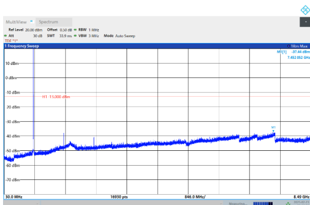
Band26-5MHz-QPSK-26815-1RB#0-Range:30~8490MHz
