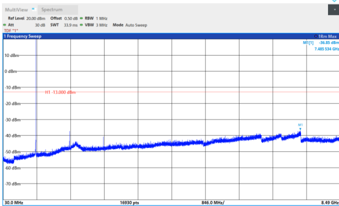
Band26-3MHz-QPSK-26915-1RB#0-Range:30~8490MHz
