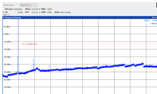
Band26-10MHz-QPSK-26840-1RB#0-Range:30~8490MHz
