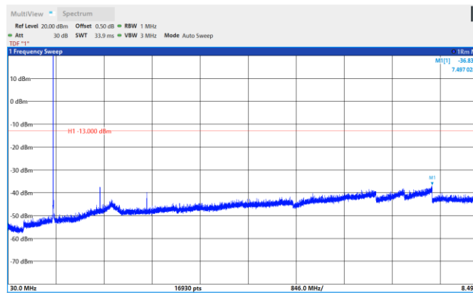
Band26-3MHz-QPSK-27025-1RB#0-Range:30~8490MHz
