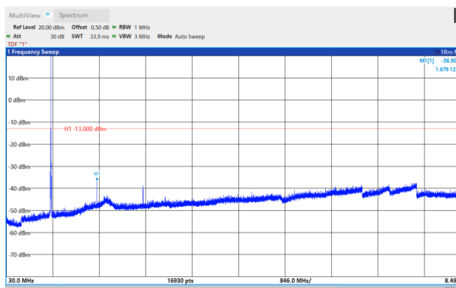
Band26-15MHz-QPSK-26915-1RB#0-Range:30~8490MHz
