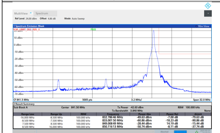
Band26-15MHz-256QAM-26865-1RB#0
