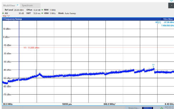
Band26-10MHz-QPSK-26915-1RB#0-Range:30~8490MHz
