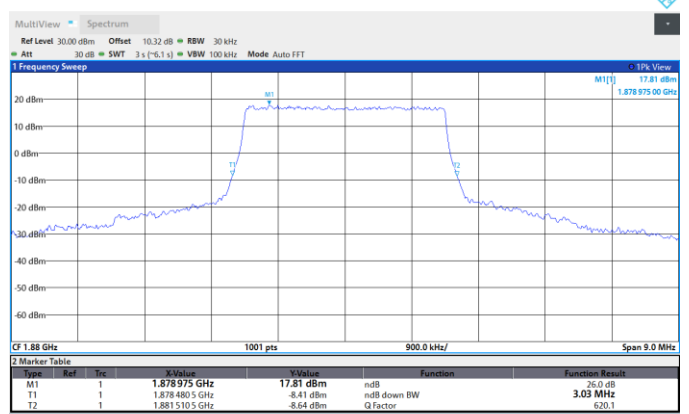
Band2-5MHz-16QAM-18900-25RB#0
