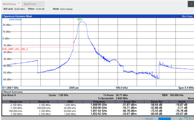
Band2-1.4MHz-64QAM-18607-1RB#0
