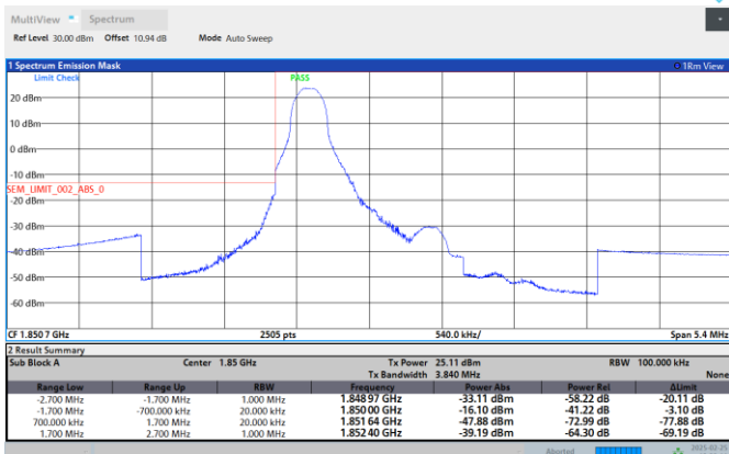
Band2-1.4MHz-16QAM-18607-1RB#0
