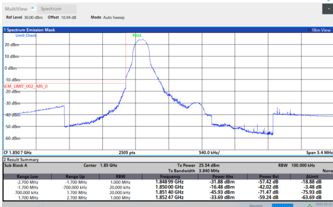
Band2-1.4MHz-64QAM-18607-1RB#0
