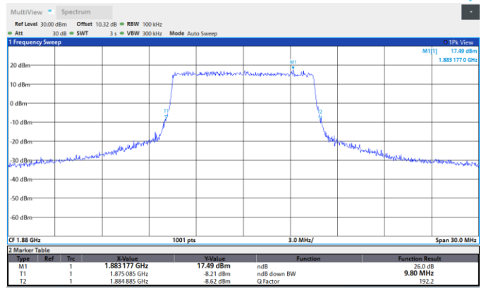
Band2-15MHz-16QAM-18900-75RB#0
