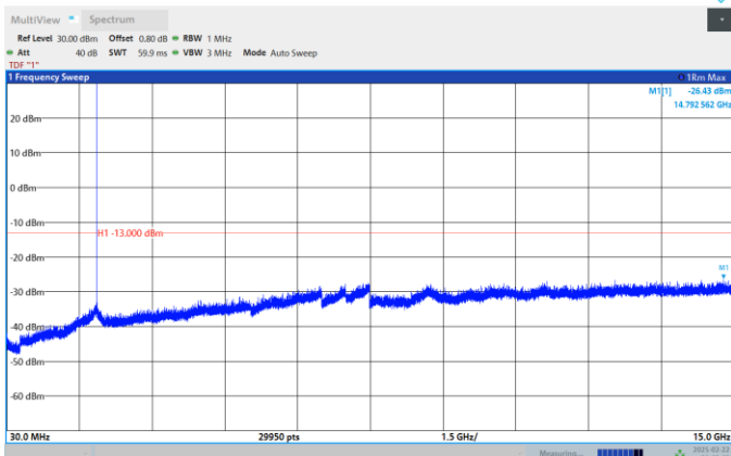
Band2-3MHz-QPSK-19185-1RB#0-Range:30~15000MHz
