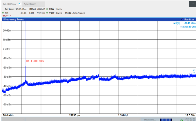
Band2-5MHz-QPSK-18900-1RB#0-Range:30~15000MHz
