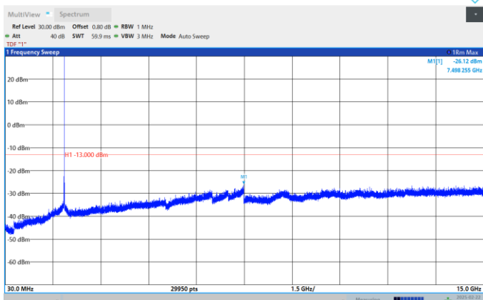
Band2-10MHz-QPSK-19150-1RB#0-Range:30~15000MHz
