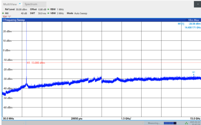
Band2-10MHz-QPSK-18900-1RB#0-Range:30~15000MHz
