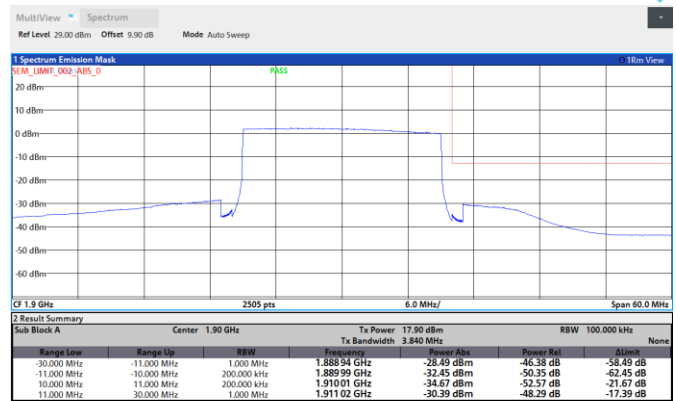
Band2-20MHz-256QAM-18700-100RB#0
