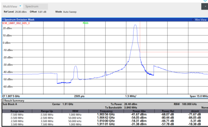
Band2-5MHz-64QAM-18625-1RB#0
