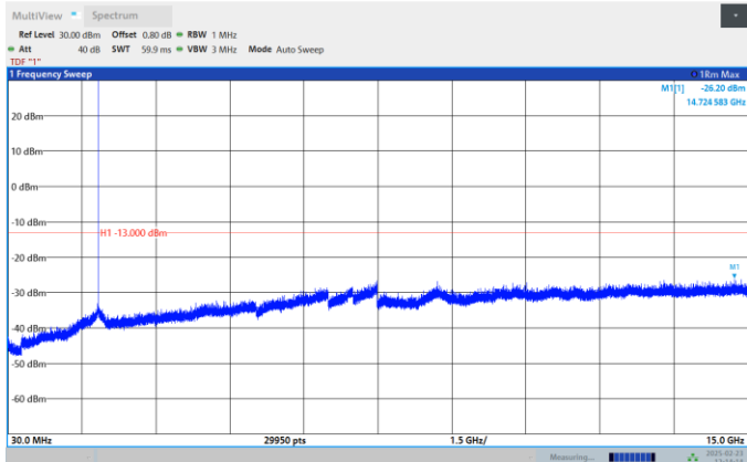
Band2-1.4MHz-QPSK-18900-1RB#0-Range:30~15000MHz
