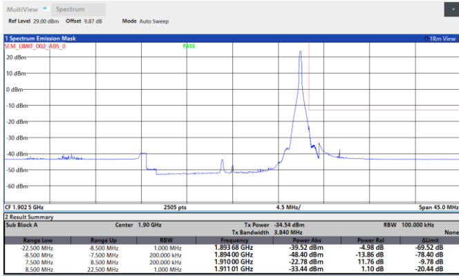
Band2-15MHz-64QAM-18675-1RB#0
