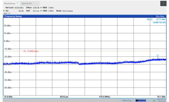
Band2-10MHz-QPSK-18900-1RB#0- Range:15000MHz~19100MHz
