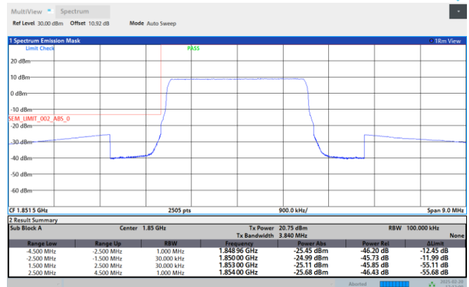
Band2-3MHz-256QAM-19185-15RB#0
