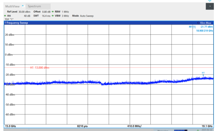
Band2-10MHz-QPSK-19150-1RB#0- Range:15000MHz~19100MHz
