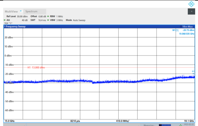
Band2-15MHz-QPSK-18675-1RB#0- Range:15000MHz~19100MHz
