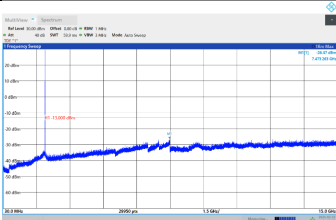
Band2-5MHz-QPSK-18625-1RB#0-Range:30~15000MHz
