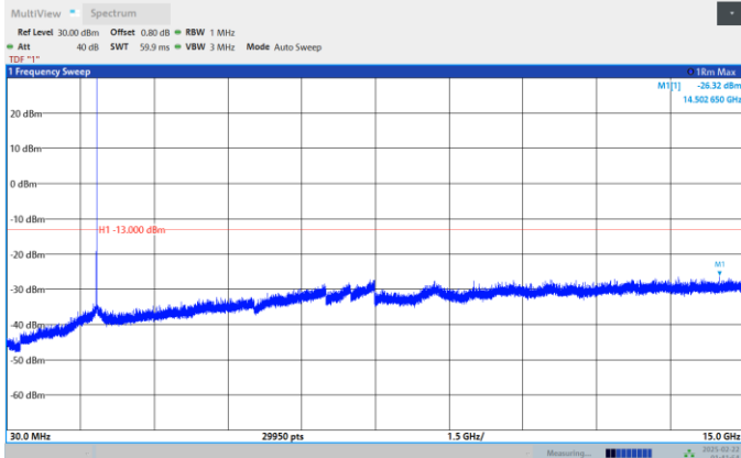
Band2-3MHz-QPSK-18900-1RB#0-Range:30~15000MHz
