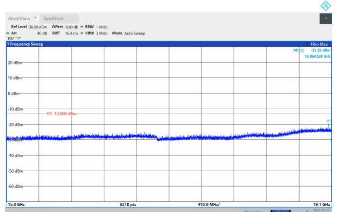
Band2-10MHz-QPSK-18650-1RB#0- Range:15000MHz~19100MHz
