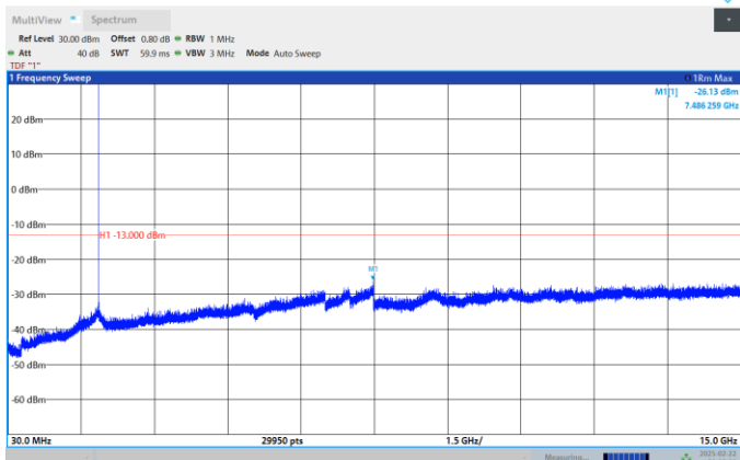
Band2-1.4MHz-QPSK-19193-1RB#0-Range:30~15000MHz
