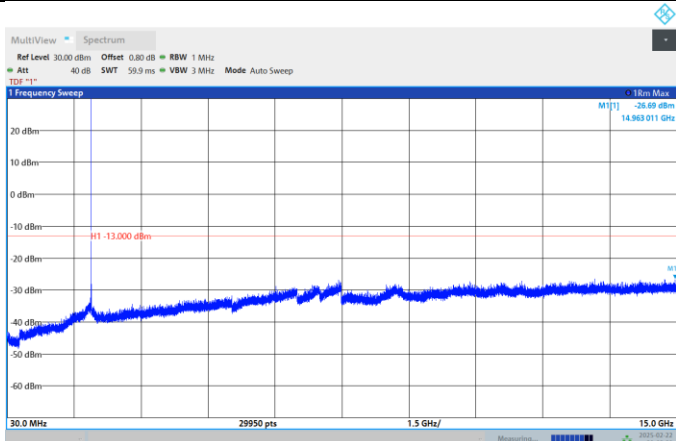
Band2-15MHz-QPSK-18675-1RB#0-Range:30~15000MHz
