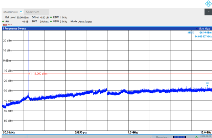
Band2-3MHz-QPSK-18615-1RB#0-Range:30~15000MHz
