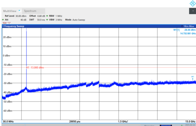
Band2-10MHz-QPSK-18650-1RB#0-Range:30~15000MHz
