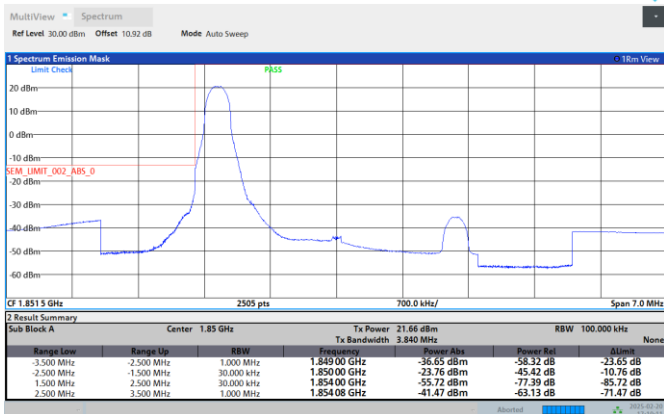
Band2-3MHz-256QAM-19185-1RB#14
