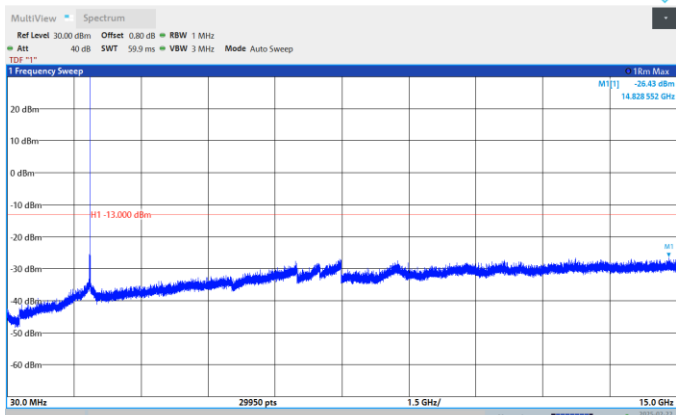
Band2-5MHz-QPSK-19175-1RB#0-Range:30~15000MHz
