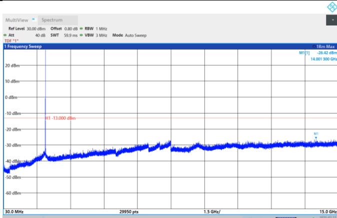
Band2-20MHz-QPSK-18700-1RB#0-Range:30~15000MHz
