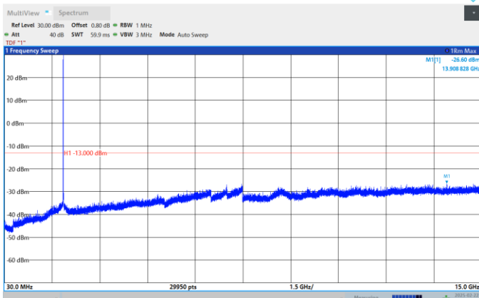
Band2-20MHz-QPSK-19100-1RB#0-Range:30~15000MHz
