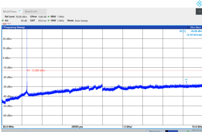
Band2-20MHz-QPSK-19100-1RB#0-Range:30~15000MHz
