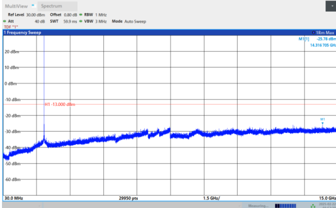
Band2-20MHz-QPSK-18900-1RB#0-Range:30~15000MHz
