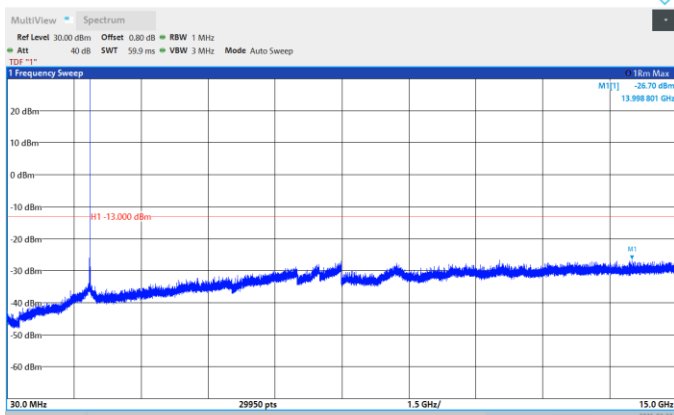
Band2-15MHz-QPSK-19125-1RB#0-Range:30~15000MHz
