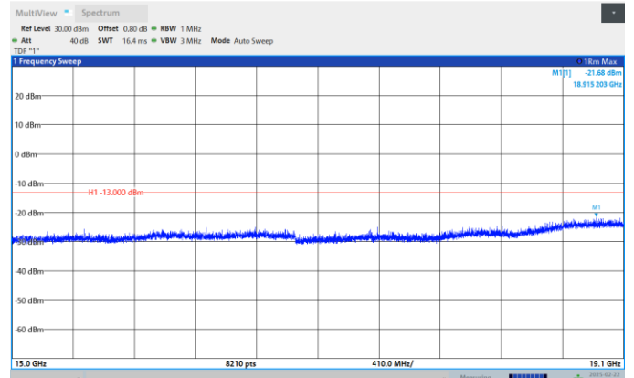
Band2-15MHz-QPSK-18900-1RB#0- Range:15000MHz~19100MHz
