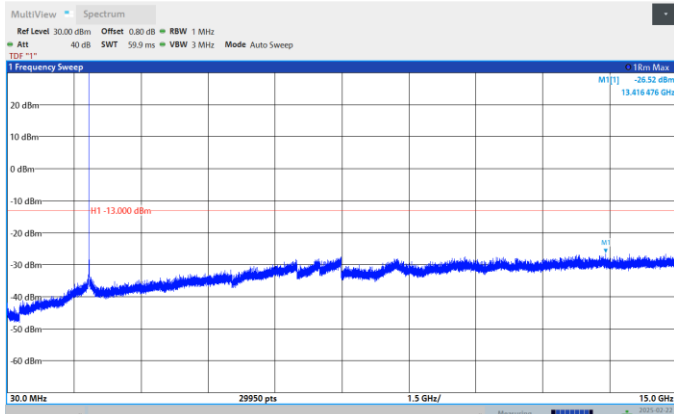
Band2-15MHz-QPSK-18900-1RB#0-Range:30~15000MHz
