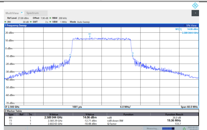
Band41-20MHz-16QAM-40620-100RB#0
