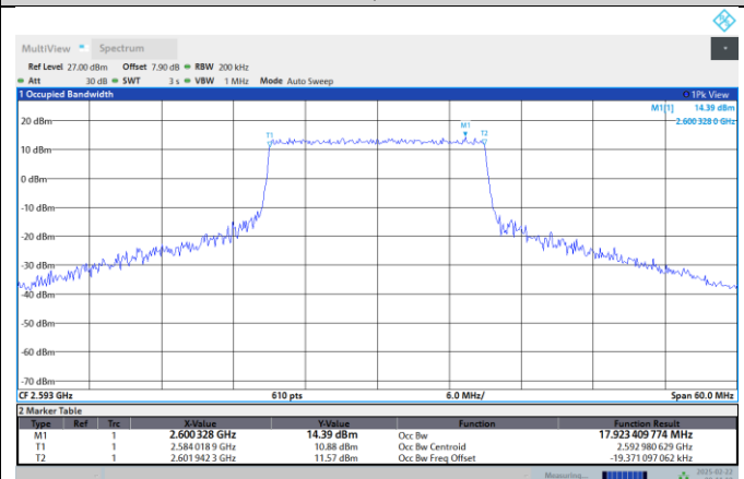
Band41-20MHz-16QAM-40620-100RB#0
