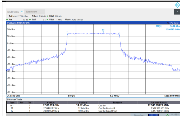
Band41-20MHz-QPSK-40620-100RB#0
