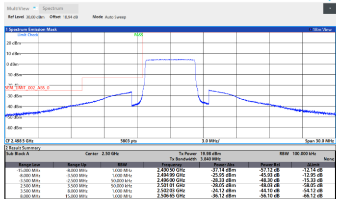
Band41-5MHz-64QAM-41565-25RB#0
