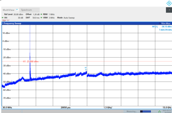
Band41-15MHz-QPSK-40620-1RB#0-Range:30~15000MHz
