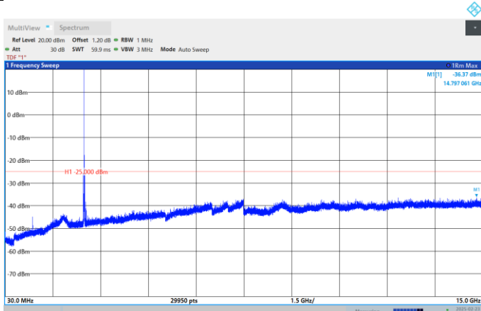
Band41-20MHz-QPSK-40620-1RB#0-Range:30~15000MHz
