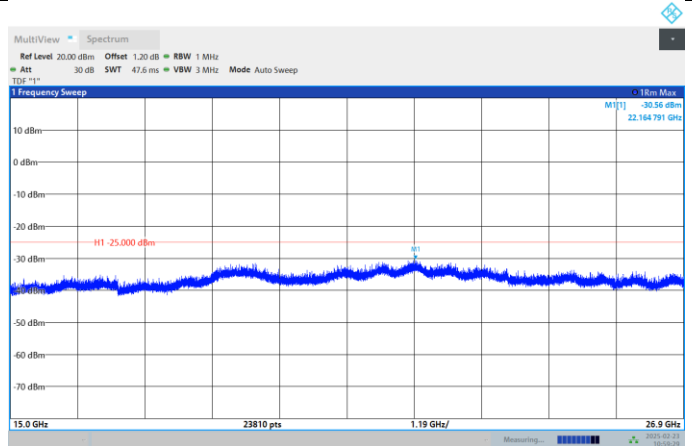
Band41-15MHz-QPSK-40620-1RB#0- Range:15000~26900MHz
