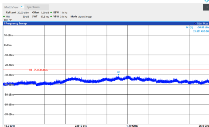
Band41-10MHz-QPSK-40620-1RB#0- Range:15000~26900MHz
