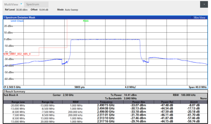
Band41-15MHz-64QAM-41515-75RB#0
