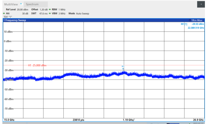
Band41-15MHz-QPSK-41515-1RB#0- Range:15000~26900MHz
