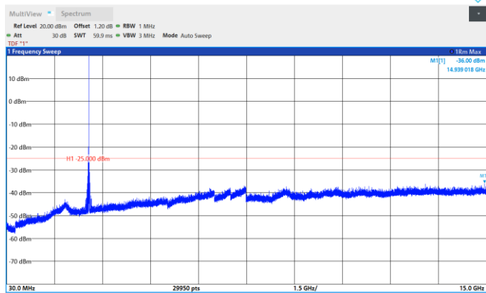
Band41-5MHz-QPSK-41565-1RB#0-Range:30~15000MHz
