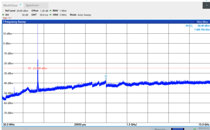
Band41-20MHz-QPSK-41490-1RB#0-Range:30~15000MHz
