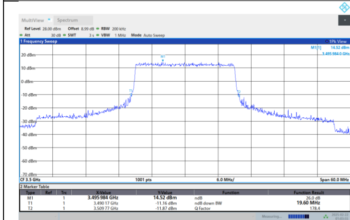
Band42-20MHz-QPSK-42590-100RB#0
