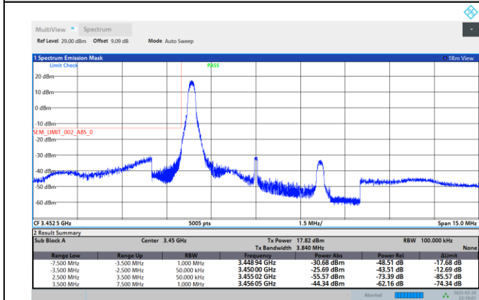
Band42-5MHz-256QAM-43065-1RB#24
