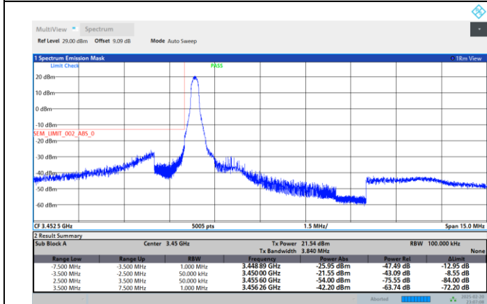
Band42-5MHz-64QAM-43065-1RB#24
