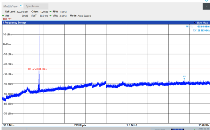
Band41-15MHz-QPSK-39725-1RB#0-Range:30~15000MHz
