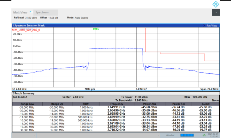
Band41-20MHz-256QAM-41490-100RB#0
