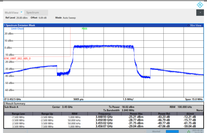
Band42-256QAM-QPSK-43065-25RB#0
