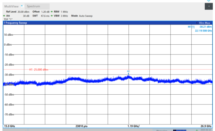
Band41-15MHz-QPSK-39725-1RB#0- Range:15000~26900MHz
