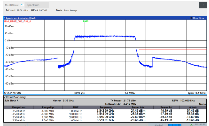
Band42-5MHz-16QAM-42115-25RB#0
