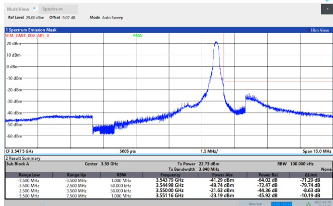
Band42-5MHz-16QAM-42115-1RB#0
