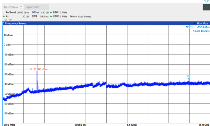
Band41-10MHz-QPSK-40620-1RB#0-Range:30~15000MHz
