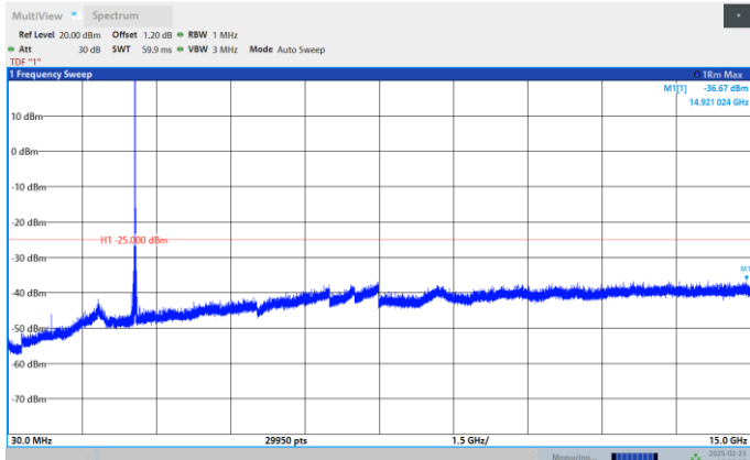
Band41-10MHz-QPSK-41540-1RB#0-Range:30~15000MHz
