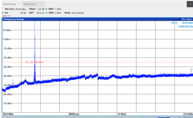
Band41-15MHz-QPSK-41515-1RB#0-Range:30~15000MHz
