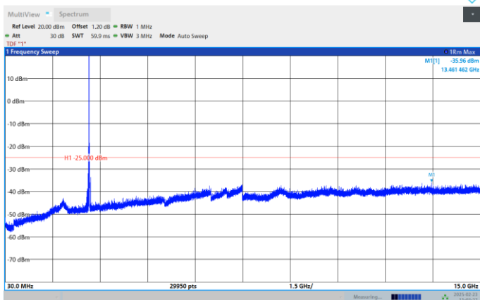
Band41-20MHz-QPSK-41490-1RB#0-Range:30~15000MHz
