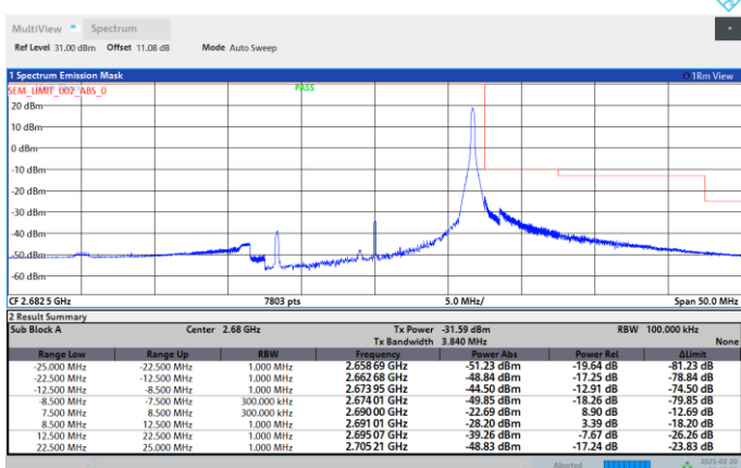
Band41-15MHz-256QAM-39725-1RB#0
