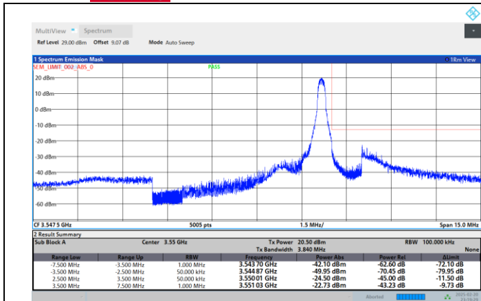
Band42-5MHz-256QAM-42115-1RB#0
