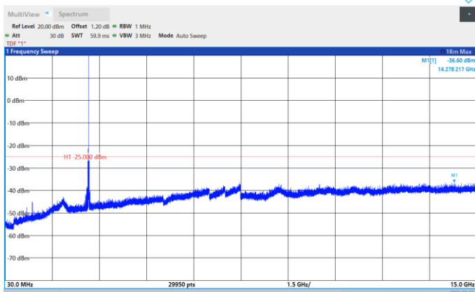
Band41-20MHz-QPSK-39750-1RB#0-Range:30~15000MHz
