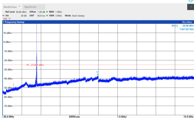
Band41-10MHz-QPSK-39700-1RB#0-Range:30~15000MHz
