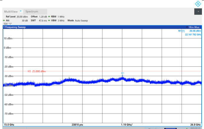
Band41-20MHz-QPSK-40620-1RB#0- Range:15000~26900MHz
