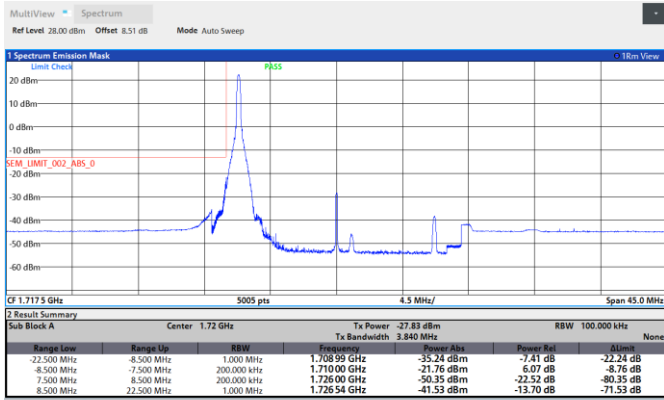
Band66-15MHz-64QAM-132597-1RB#74
