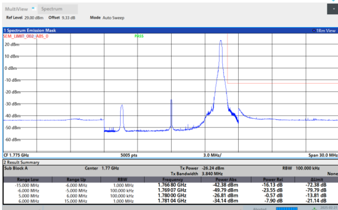
Band66-10MHz-256QAM-132022-1RB#0
