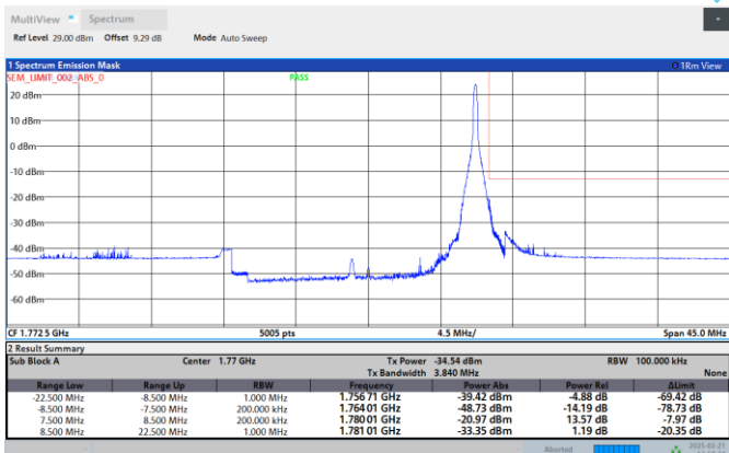
Band66-15MHz-64QAM-132047-1RB#0
