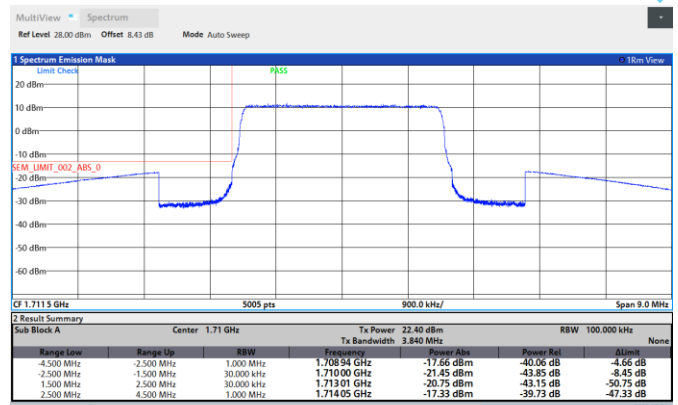
Band66-3MHz-16QAM-132657-15RB#0
