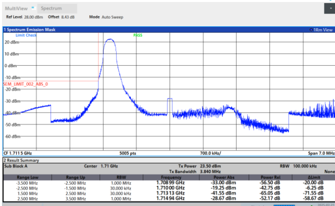
Band66-3MHz-64QAM-132657-1RB#14
