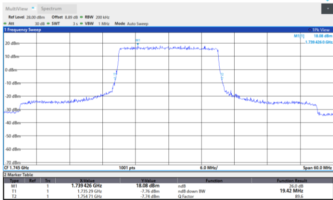
Band66-20MHz-QPSK-132322-100RB#0
