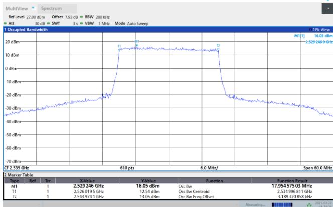
Band7-20MHz-QPSK-21100-100RB#0
