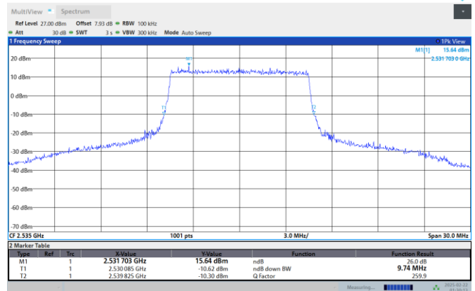
Band7-15MHz-16QAM-21100-75RB#0
