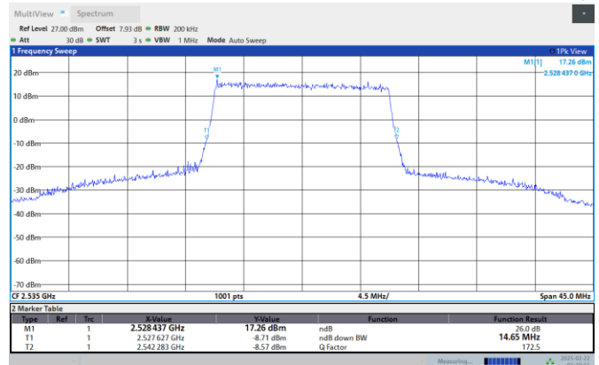
Band7-20MHz-16QAM-21100-100RB#0
