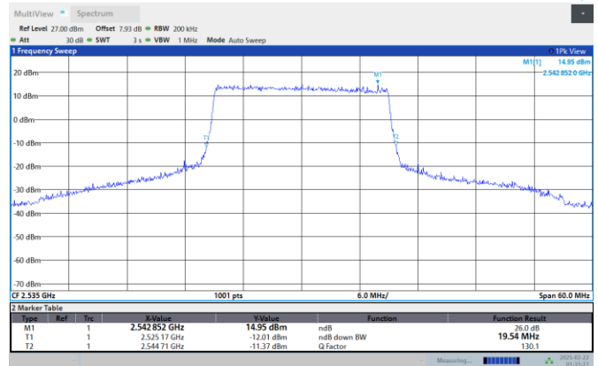
Band7-20MHz-16QAM-21100-100RB#0
