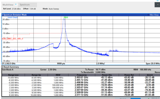
Band7-5MHz-QPSK-21425-1RB#24
