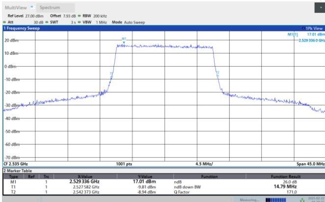
Band7-20MHz-QPSK-21100-100RB#0
