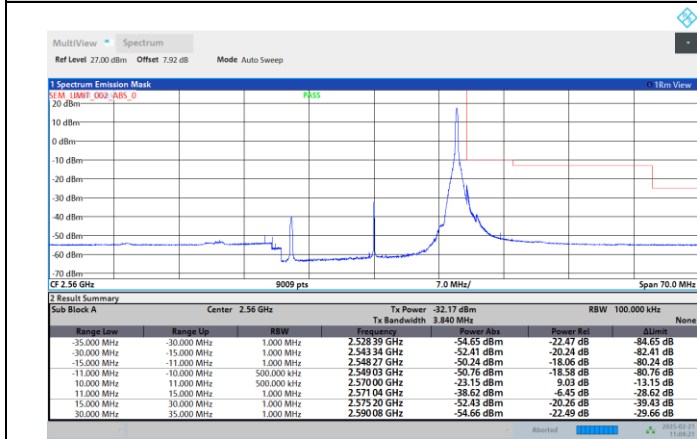
Band7-20MHz-256QAM-21350-1RB#99
