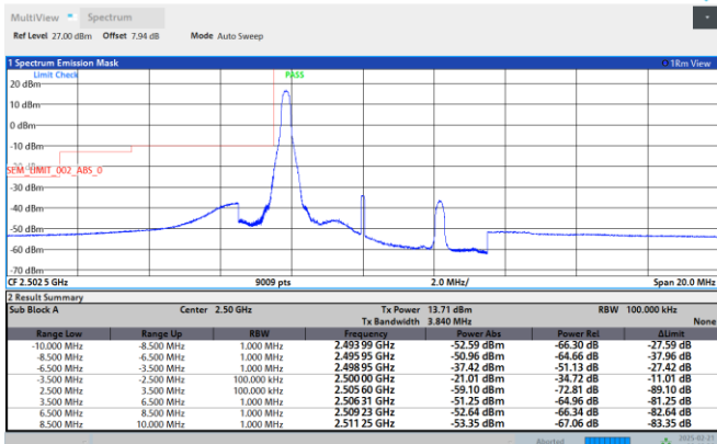
Band7-5MHz-256QAM-21425-1RB#24
