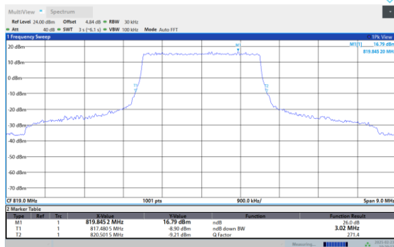
Band26-5MHz-QPSK-26740-25RB#0
