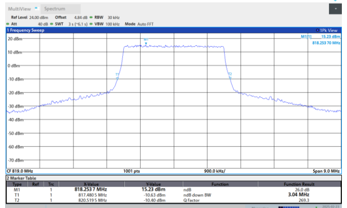
Band26-5MHz-16QAM-26740-25RB#0
