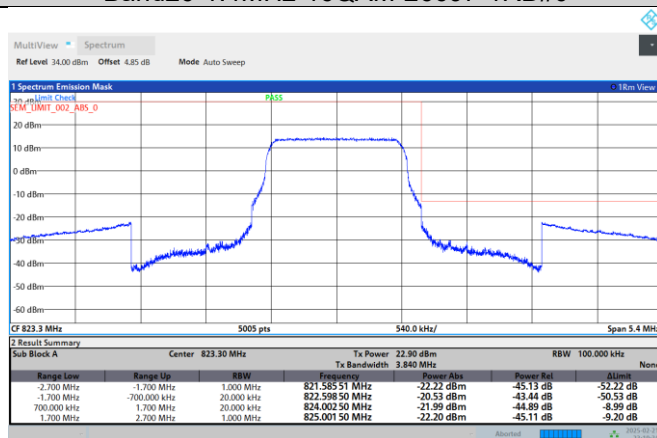
Band26-1.4MHz-16QAM-26783-1RB#5
