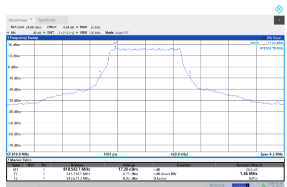
Band26-3MHz-16QAM-26740-15RB#0
