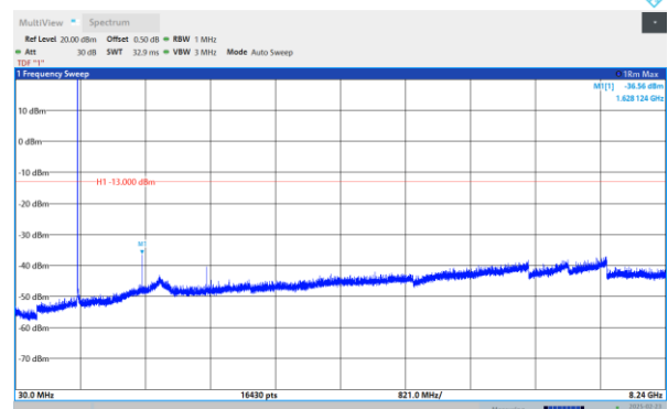
Band26-1.4MHz-QPSK-26783-1RB#0- Range1:30~8240MHz
