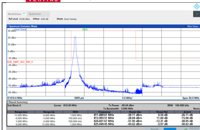
Band26-10MHz-64QAM-26740-1RB#49
