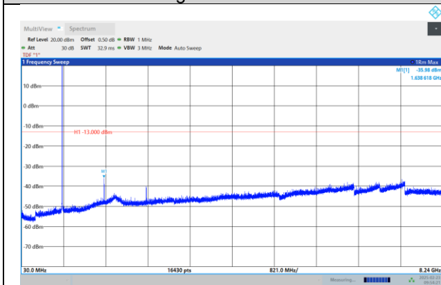
Band26-5MHz-QPSK-26765-1RB#0- Range1:30~8240MHz
