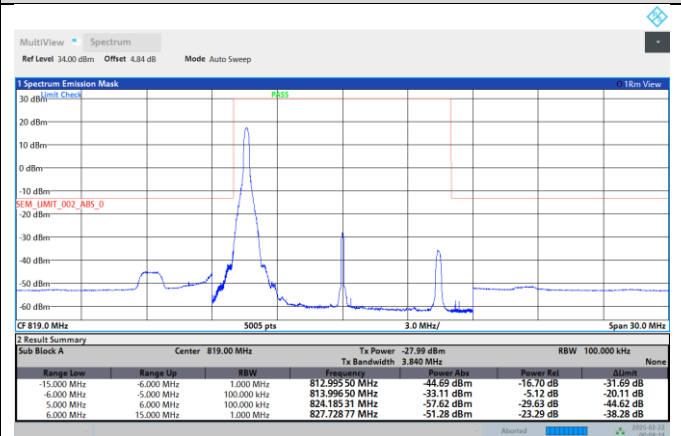
Band26-10MHz-256QAM-26740-1RB#49
