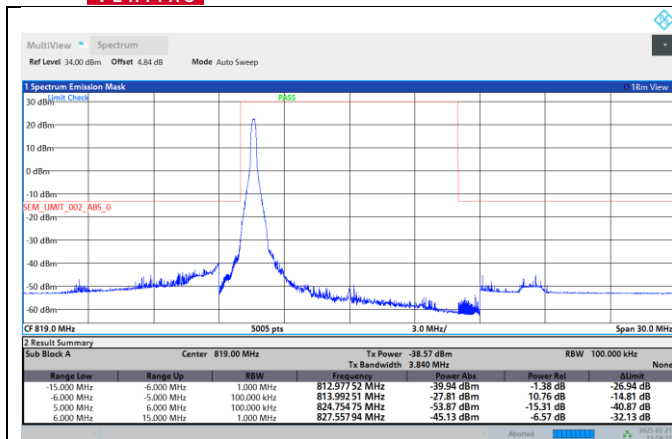
Band26-10MHz-QPSK-26740-1RB#49
