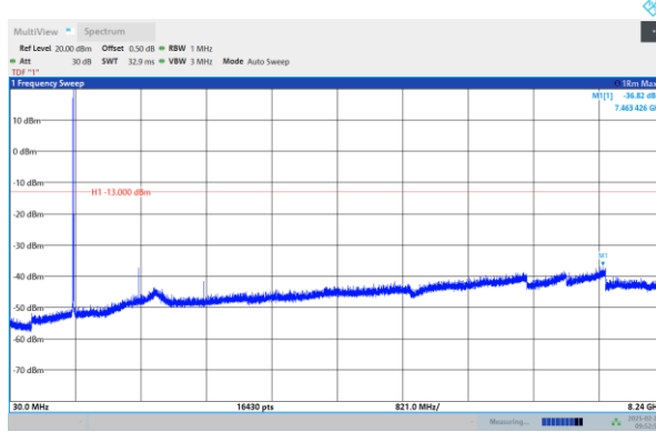
Band26-5MHz-QPSK-26740-1RB#0- Range1:30~8240MHz
