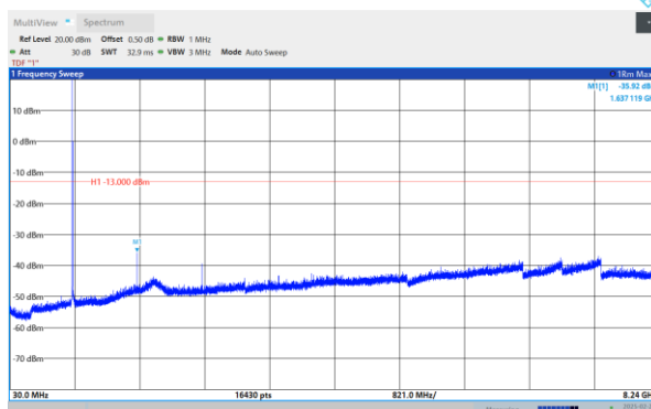
Band26-3MHz-QPSK-26705-1RB#0- Range1:30~8240MHz
