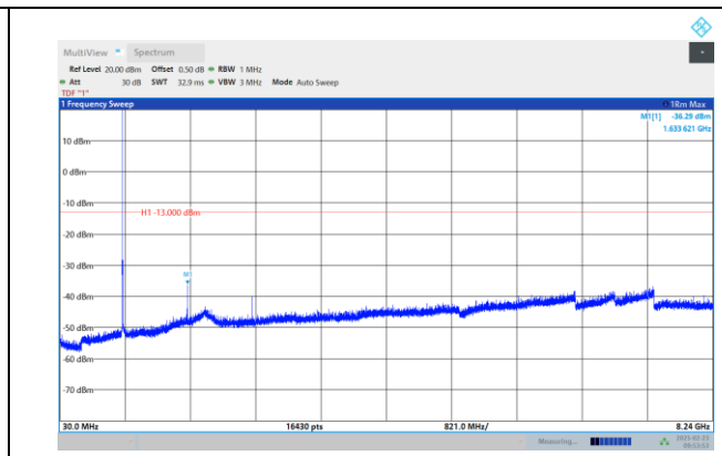
Band26-10MHz-QPSK-26740-1RB#0- Range1:30~8240MHz
