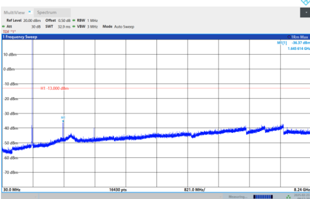
Band26-3MHz-QPSK-26740-1RB#0- Range1:30~8240MHz
