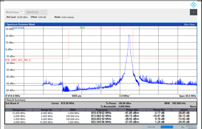
Band26-10MHz-64QAM-26740-50RB#0
