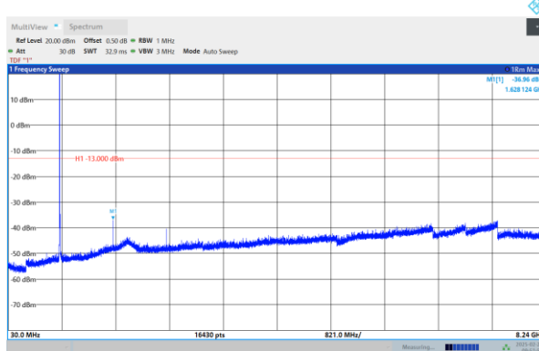
Band26-3MHz-QPSK-26775-1RB#0- Range1:30~8240MHz
