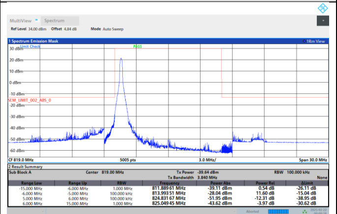
Band26-10MHz-16QAM-26740-1RB#49
