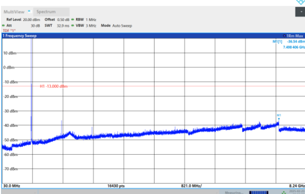
Band26-5MHz-QPSK-26715-1RB#0- Range1:30~8240MHz
